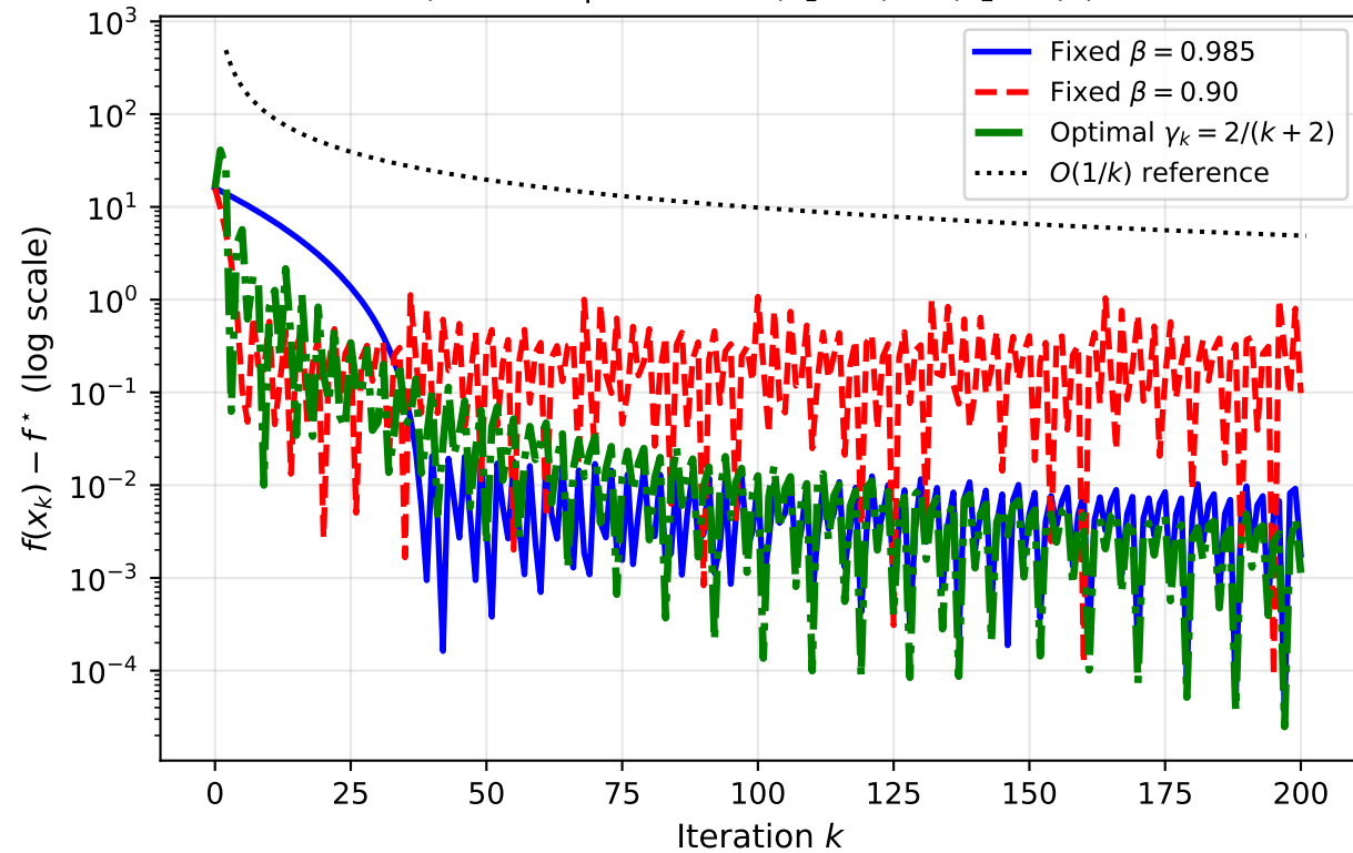
Convergence: Optimal vs Fixed- \beta Frank--Wolfe (Interior optimum f = (x_1 - 1)^2 + (x_2 - 5)^2 )
