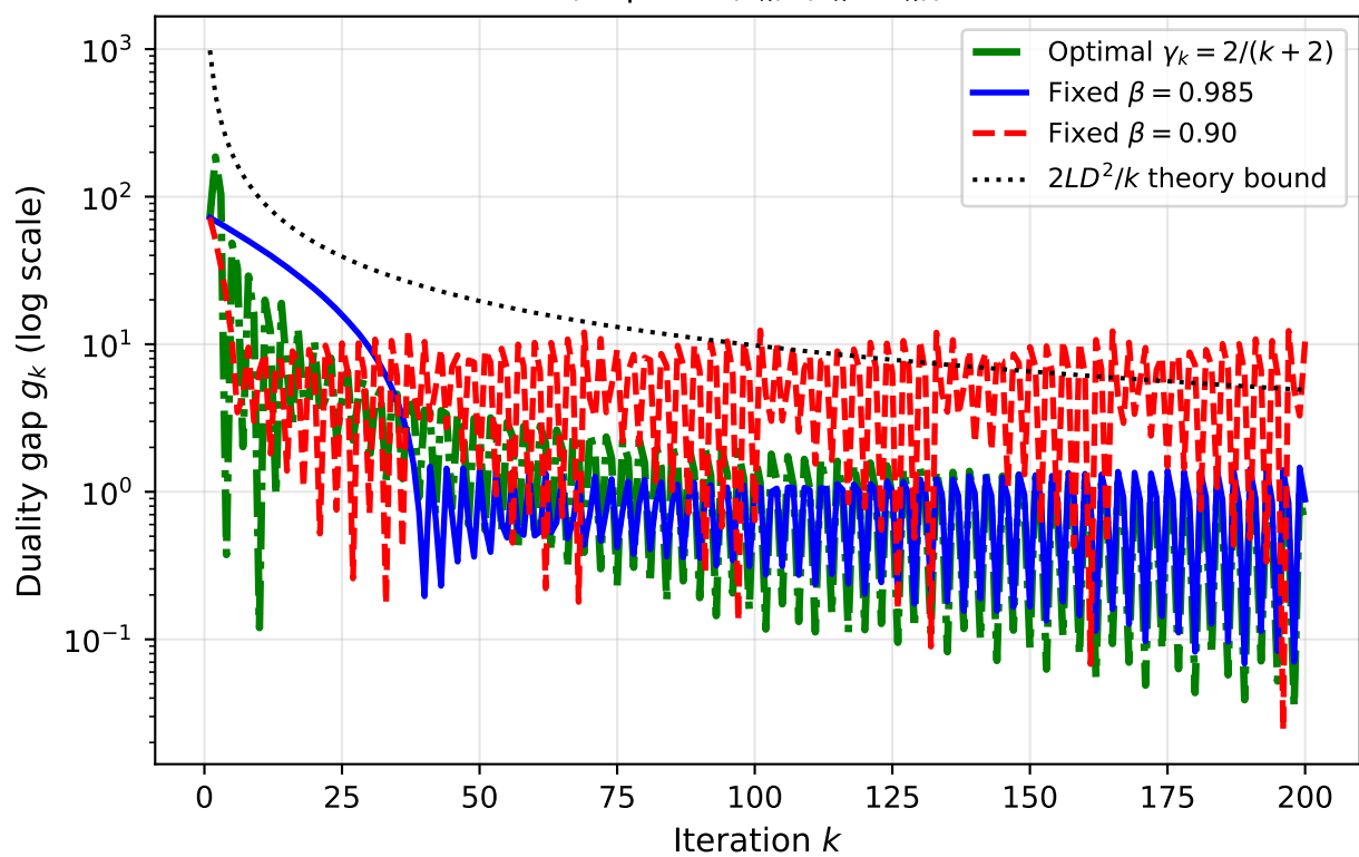
Duality Gap: Optimal vs Fixed- \beta (Gap = \nabla f(x_k)^T(x_k - z_k) )
