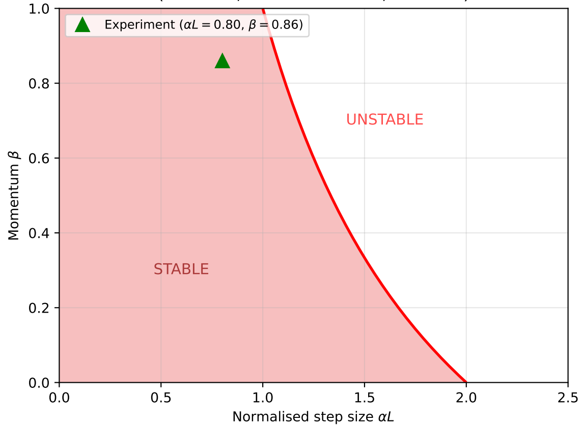
Heavy Ball Stability Region (Bench. C, L \approx 1002 at start, \kappa \approx 2505 )
