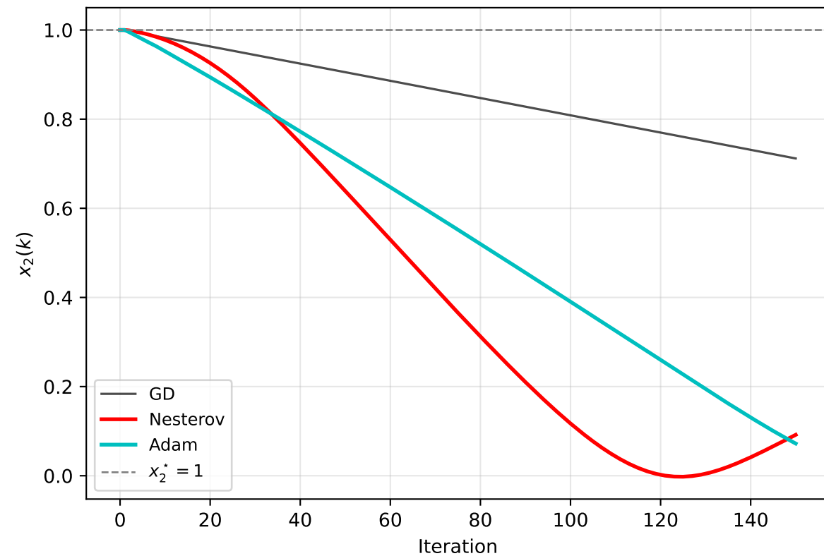
Rosenbrock trajectory (2D)
