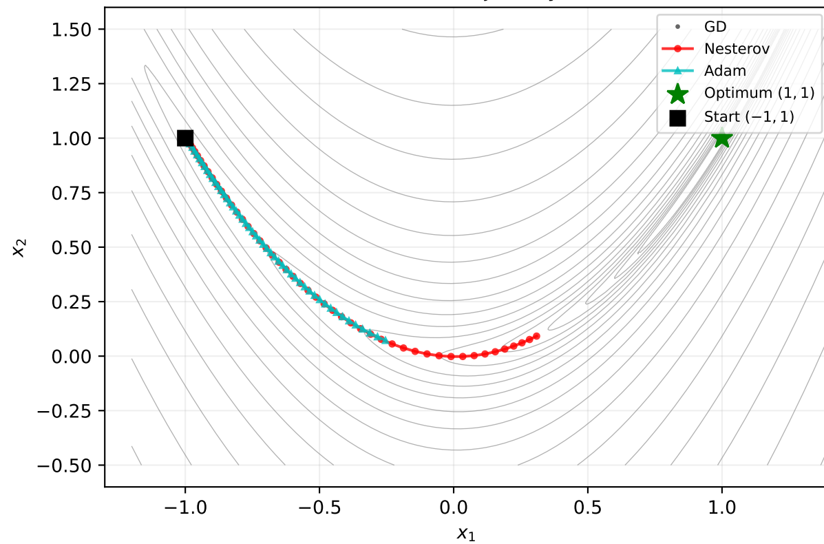
Rosenbrock trajectory (2D)
