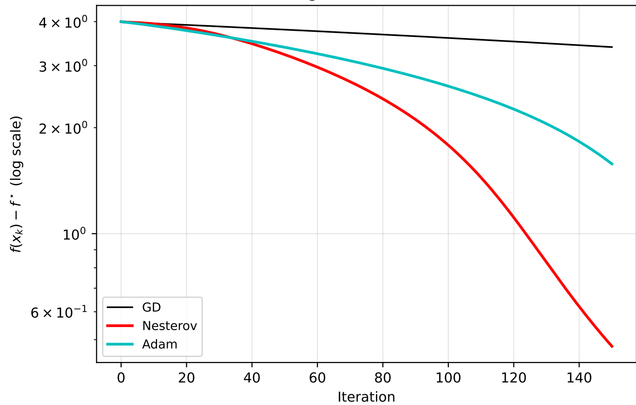
Convergence on Rosenbrock
