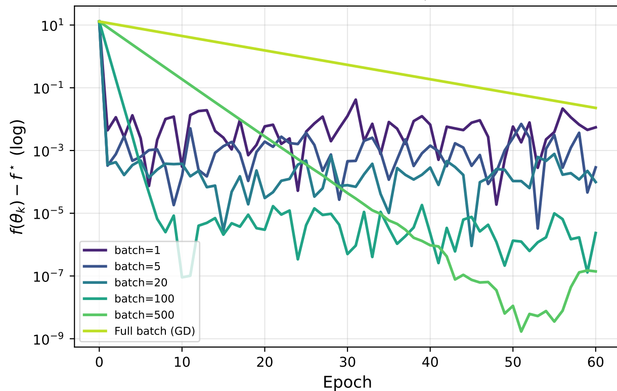
SGD Noise Floor vs Batch Size (Benchmark A, \alpha = 0.05 , 60 epochs)
