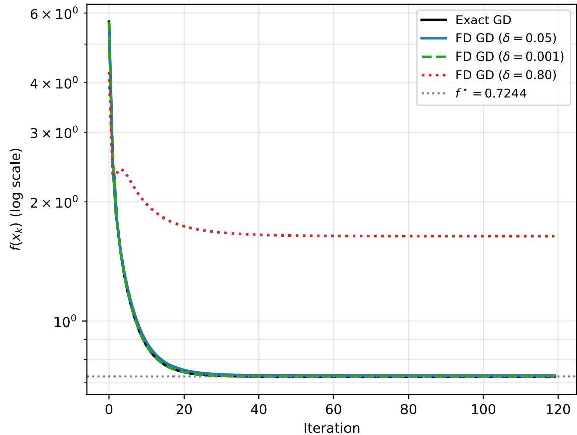
FD GD Convergence on Benchmark B
