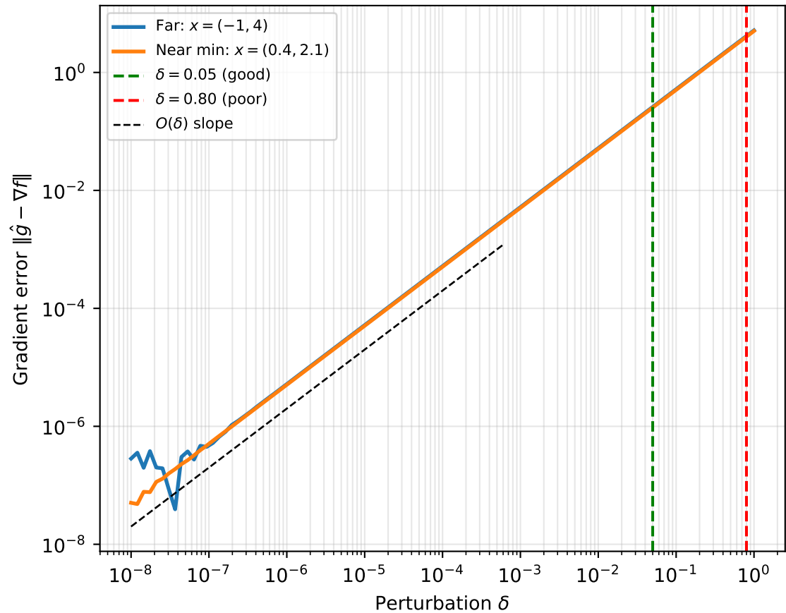
FD Gradient Error vs \delta on Benchmark B
