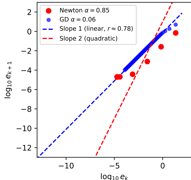
Log-Log Convergence Plot (slope 2 = quadratic convergence)
