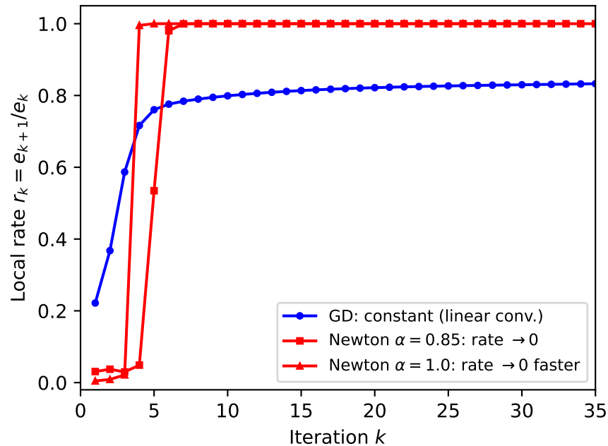
Local Convergence Rate Over Iterations (0 = perfect; 1 = no progress)
