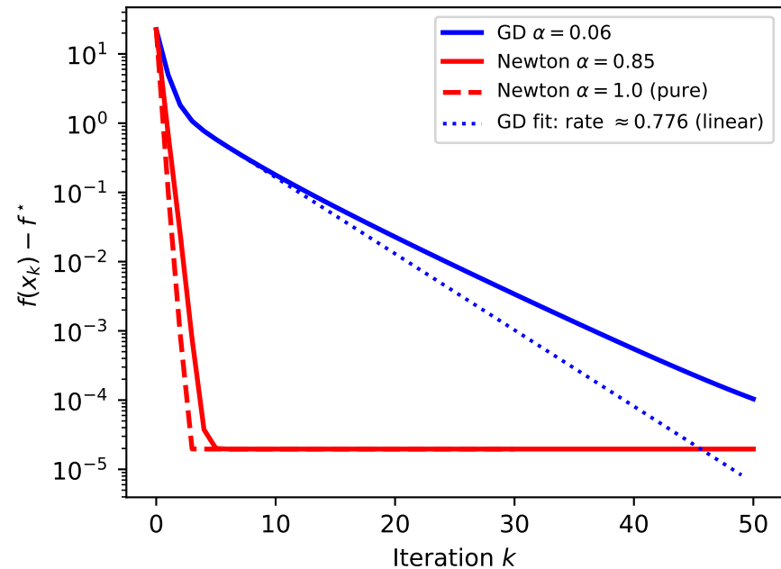
Newton vs GD Convergence (Benchmark B, 50 iters)
