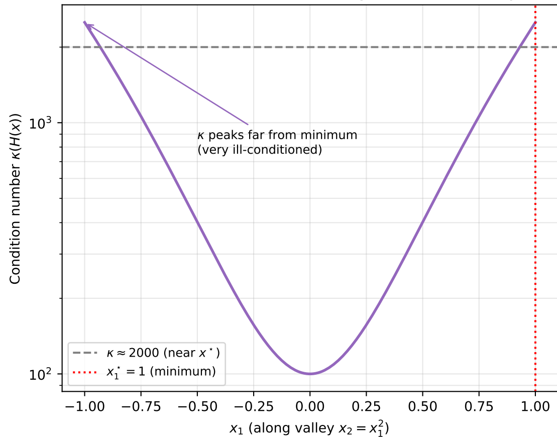
Hessian Condition Number Along Rosenbrock Valley
