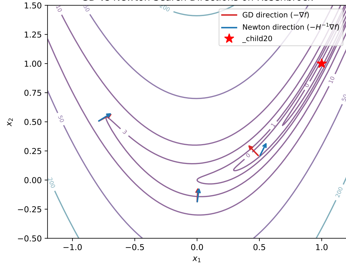
GD vs Newton Search Directions on Rosenbrock
