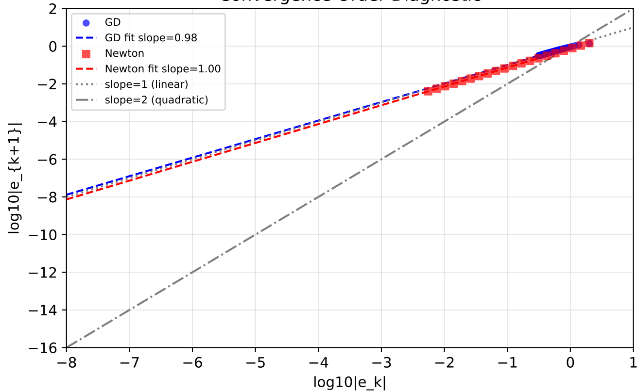
Convergence Order Diagnostic
