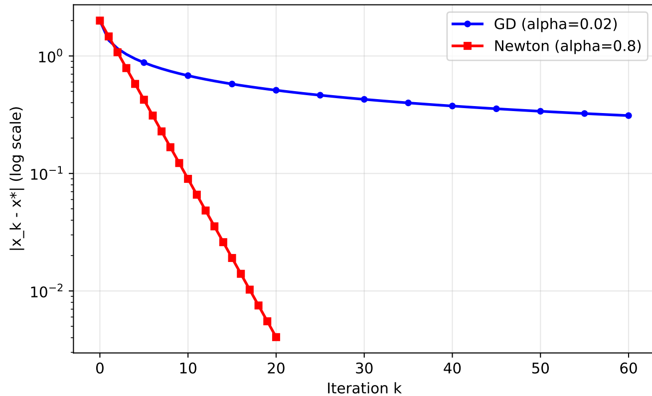
GD vs Newton on f(x)=(x-1)^4
