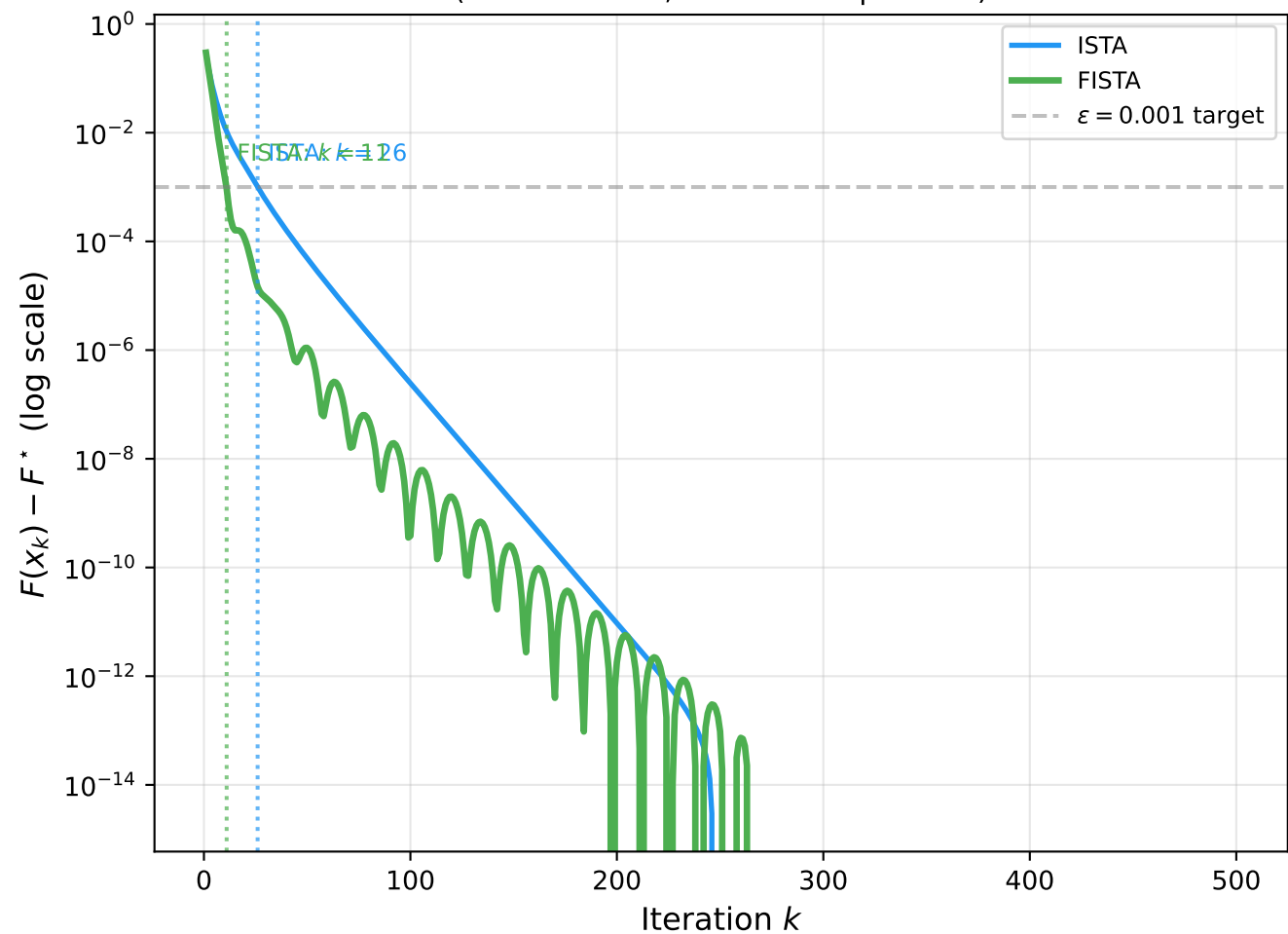
ISTA vs FISTA: Iterations to \varepsilon -Accuracy (500 iterations, same Lasso problem)
