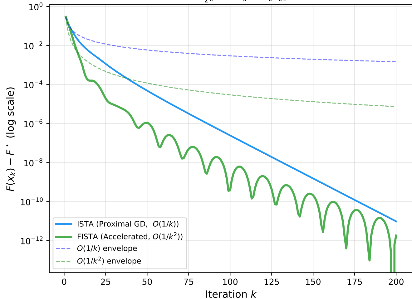
ISTA vs FISTA on Lasso-type Objective
