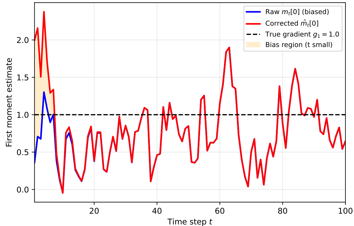
Adam Bias Correction: First Moment m_t ( \beta_1 = 0.82 , true gradient = 1.0)
