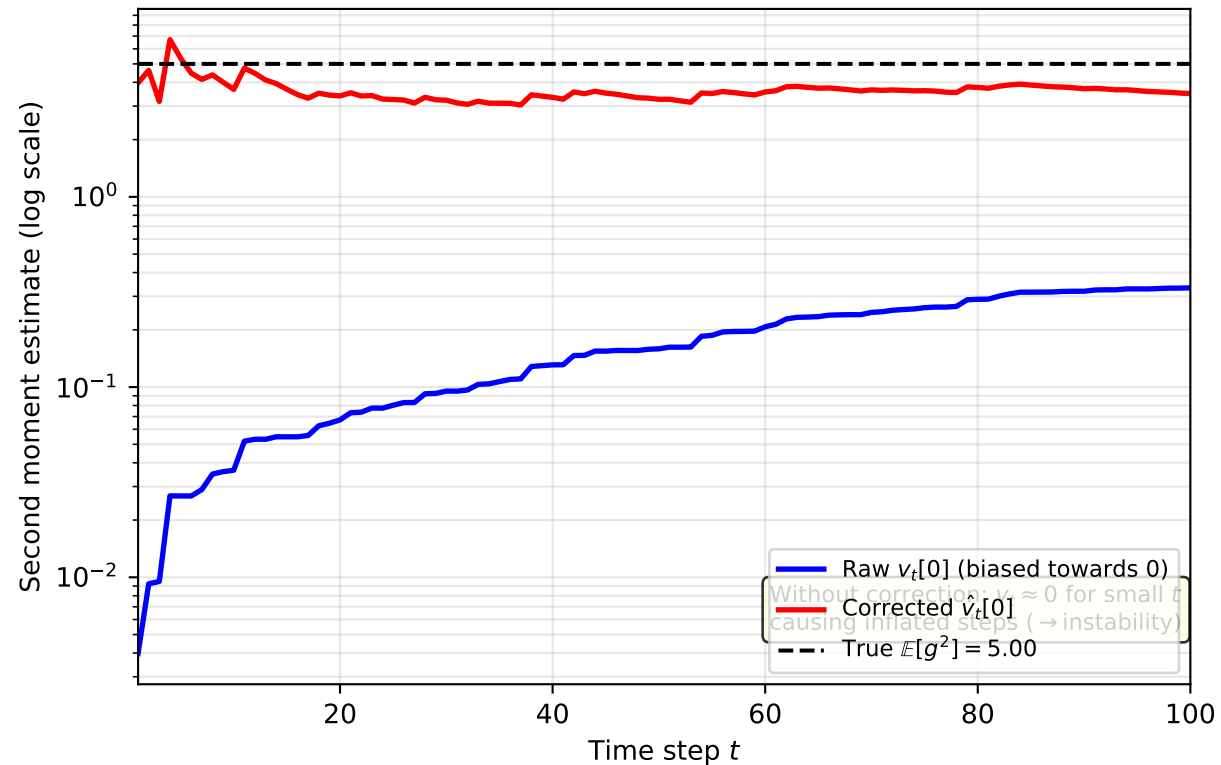
Adam Bias Correction: Second Moment v_t ( \beta_2 = 0.999 )
