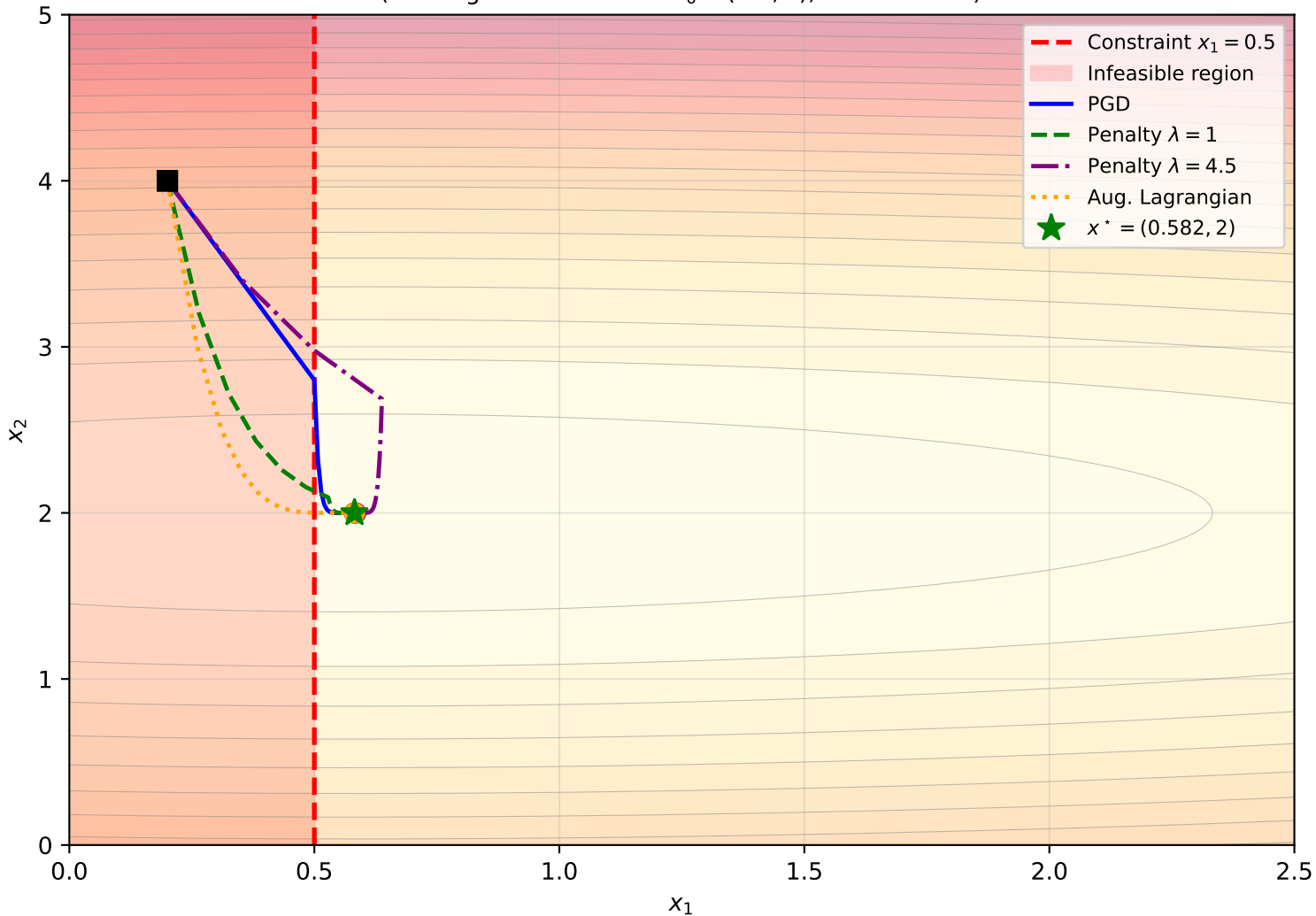
Constrained Optimisation: PGD, Penalty, Augmented Lagrangian Trajectories (starting from infeasible x_0 = (0.2, 4) , 80 iterations)
