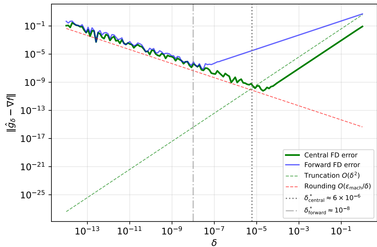
Central vs Forward Finite Differences — Benchmark B
