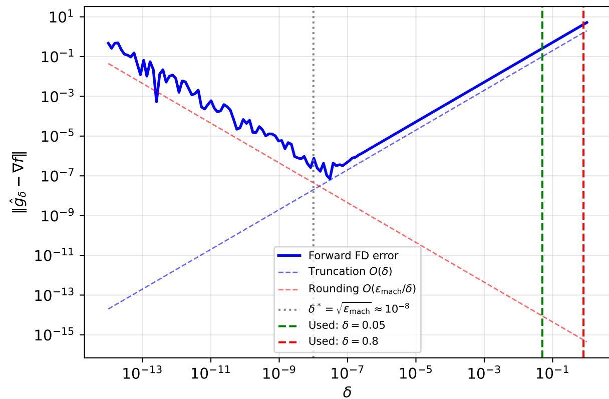
Forward Finite Differences — Benchmark B
