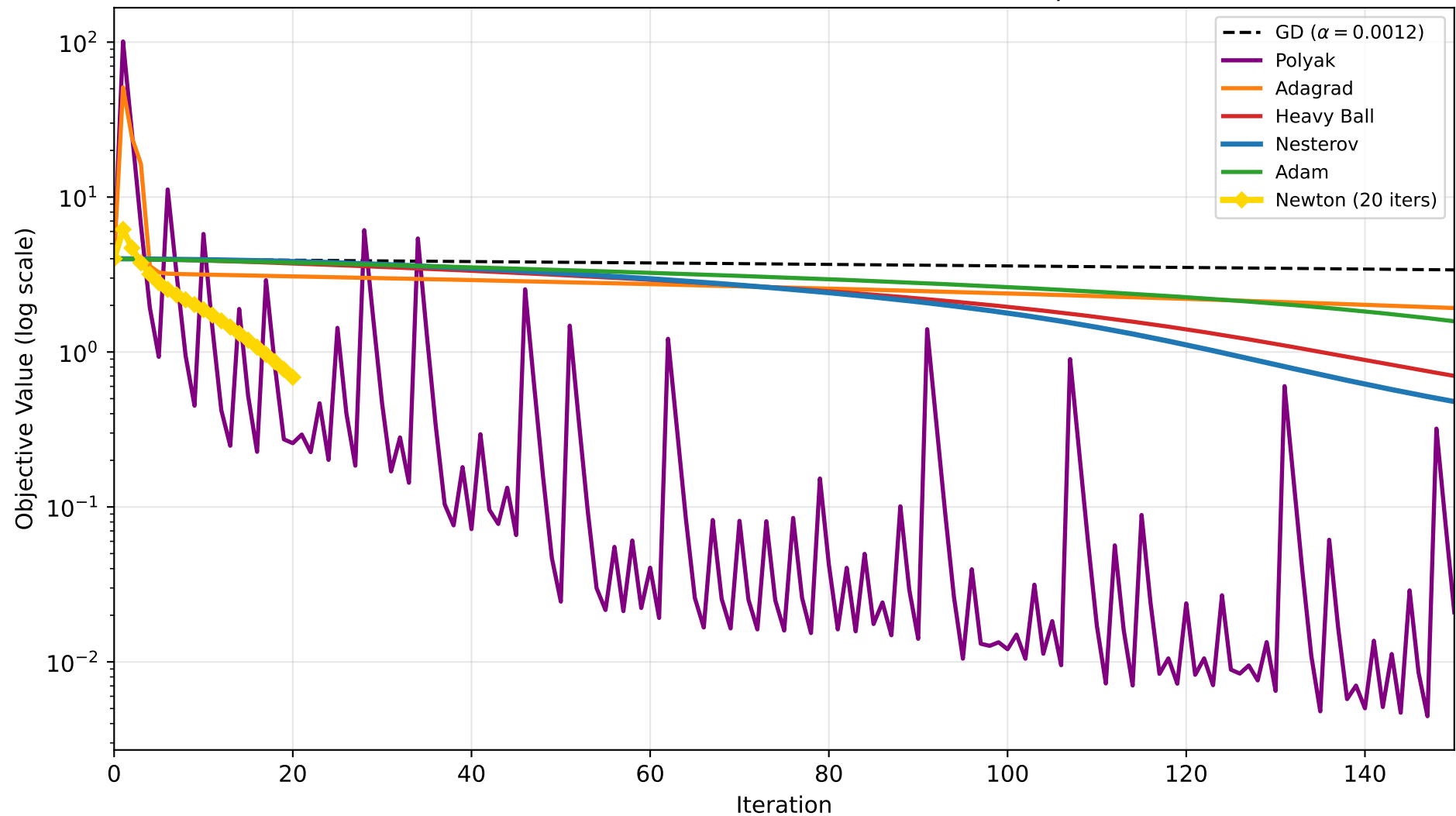
Benchmark C (Rosenbrock): All Methods Compared
