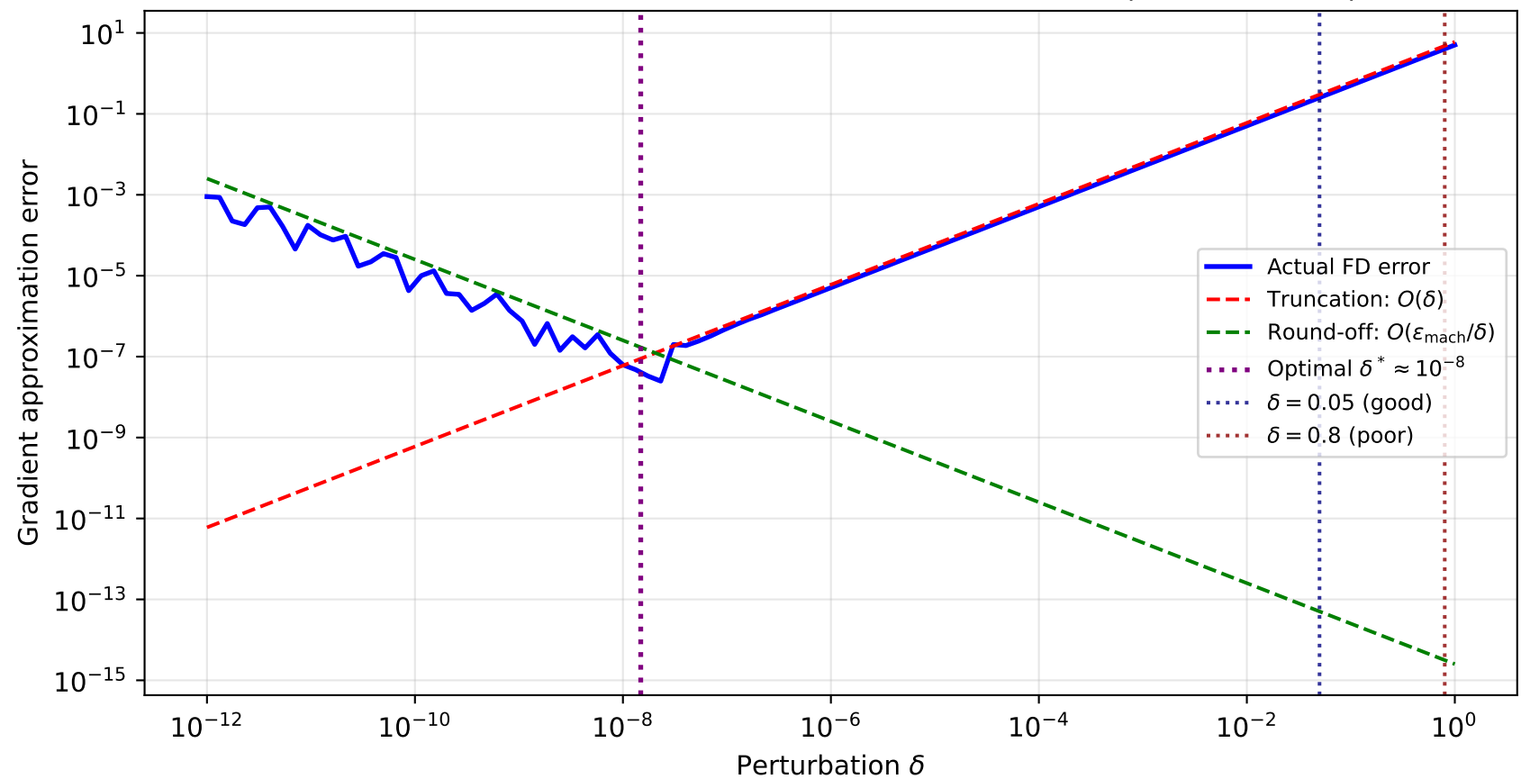
FD Gradient: Truncation vs Round-off Error Tradeoff (Benchmark B)
