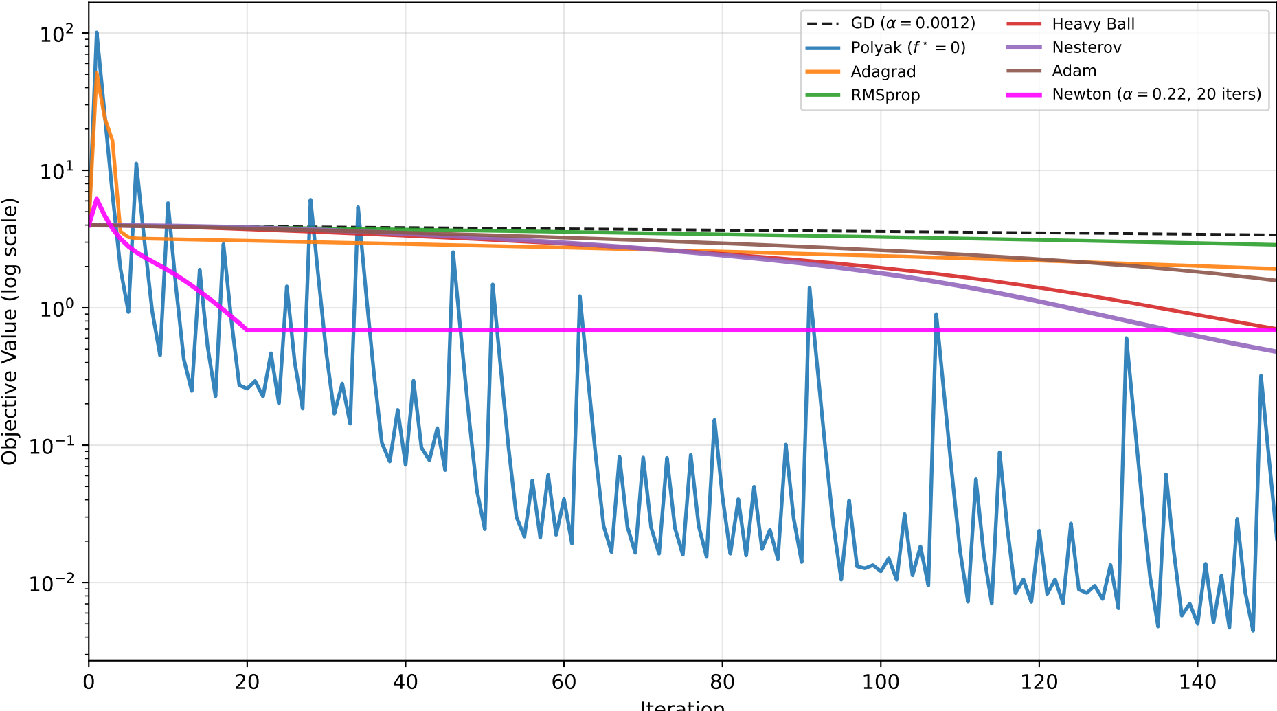
Master Convergence Comparison — Benchmark C (Rosenbrock, \kappa \approx 2504 )
