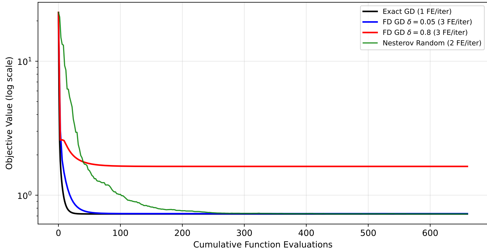
Q4: Oracle Efficiency Comparison — Benchmark B (Toy Neural Network)
