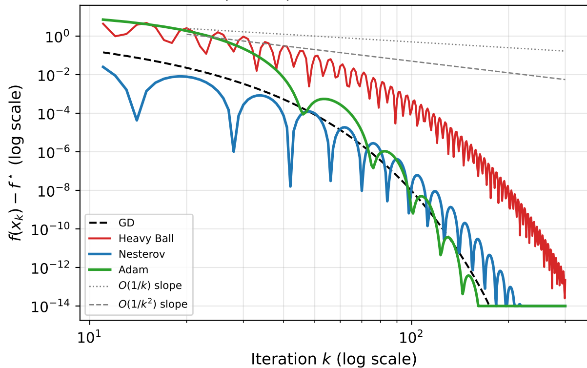
Log-Log Plot: Convergence Order (Slope = -p means O(1/k^p) rate)
