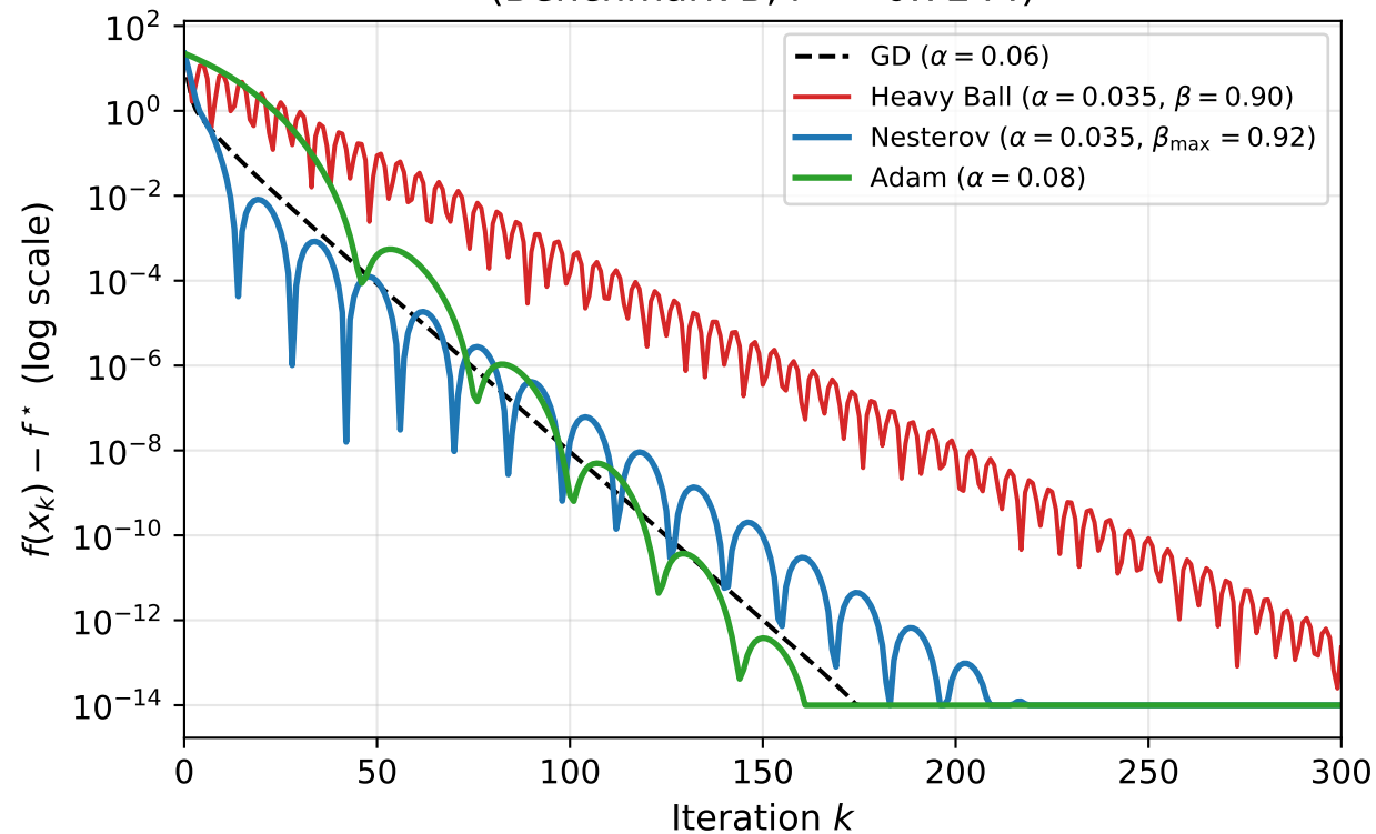
Excess Objective vs Iteration (Benchmark B, f^* = 0.7244 )
