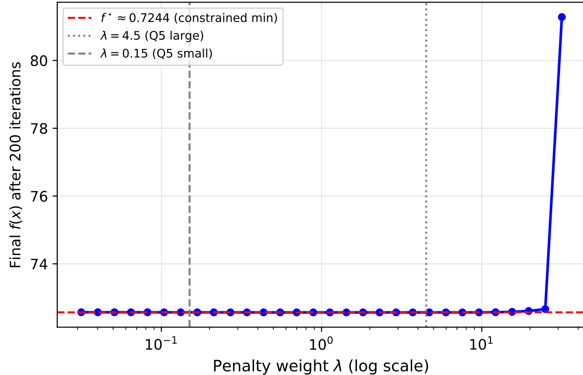
Penalty Method: Final Objective vs \lambda
