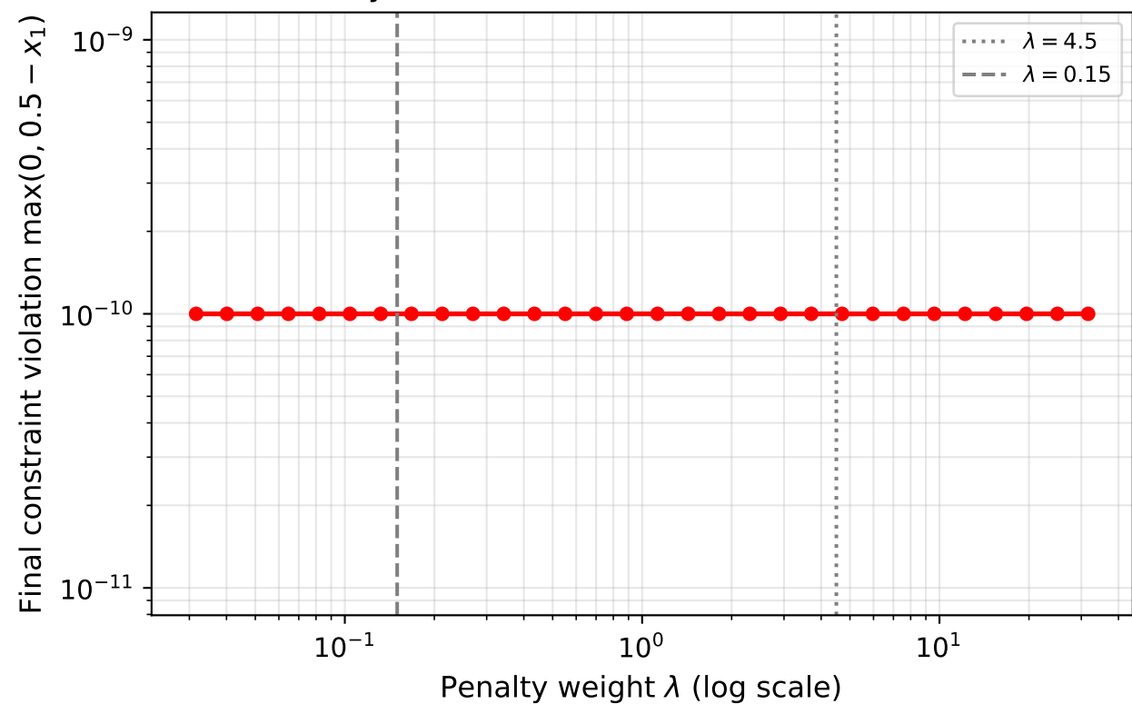
Penalty Method: Final Constraint Violation vs \lambda
