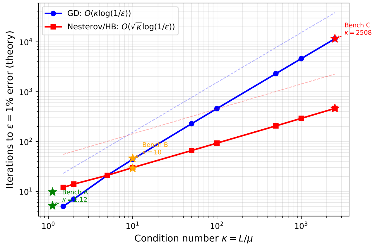
Convergence Cost vs Condition Number (strongly convex quadratic theory)
