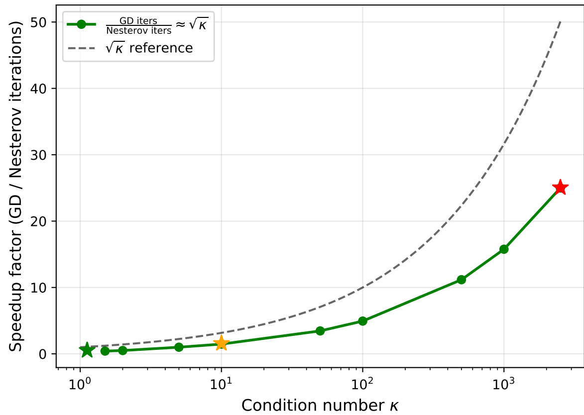
Nesterov Speedup over GD \approx \sqrt{\kappa} for strongly convex quadratics
