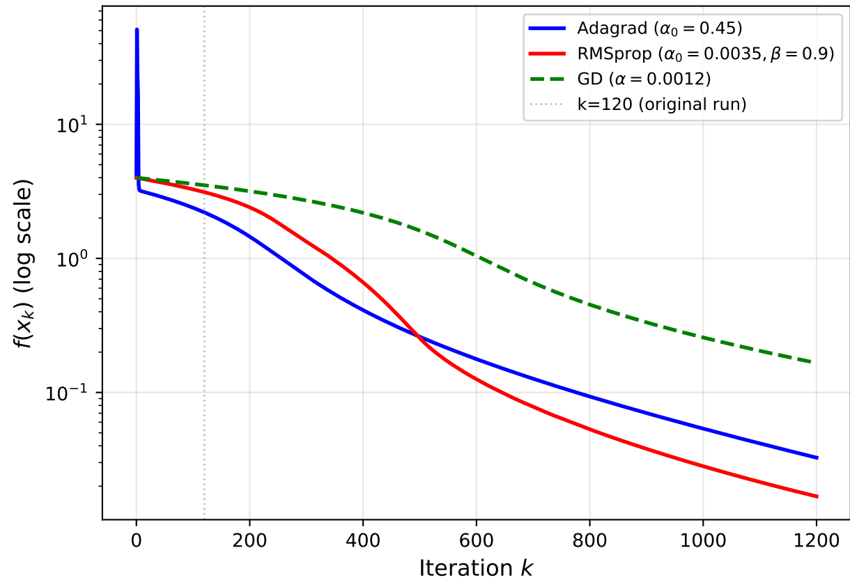
Benchmark C Rosenbrock (1200 iters): Long-run behaviour
