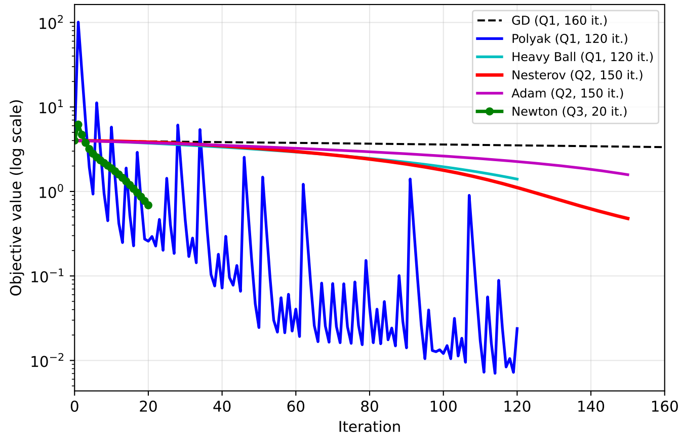
Cross-Question: All Methods on Benchmark C (Rosenbrock)
