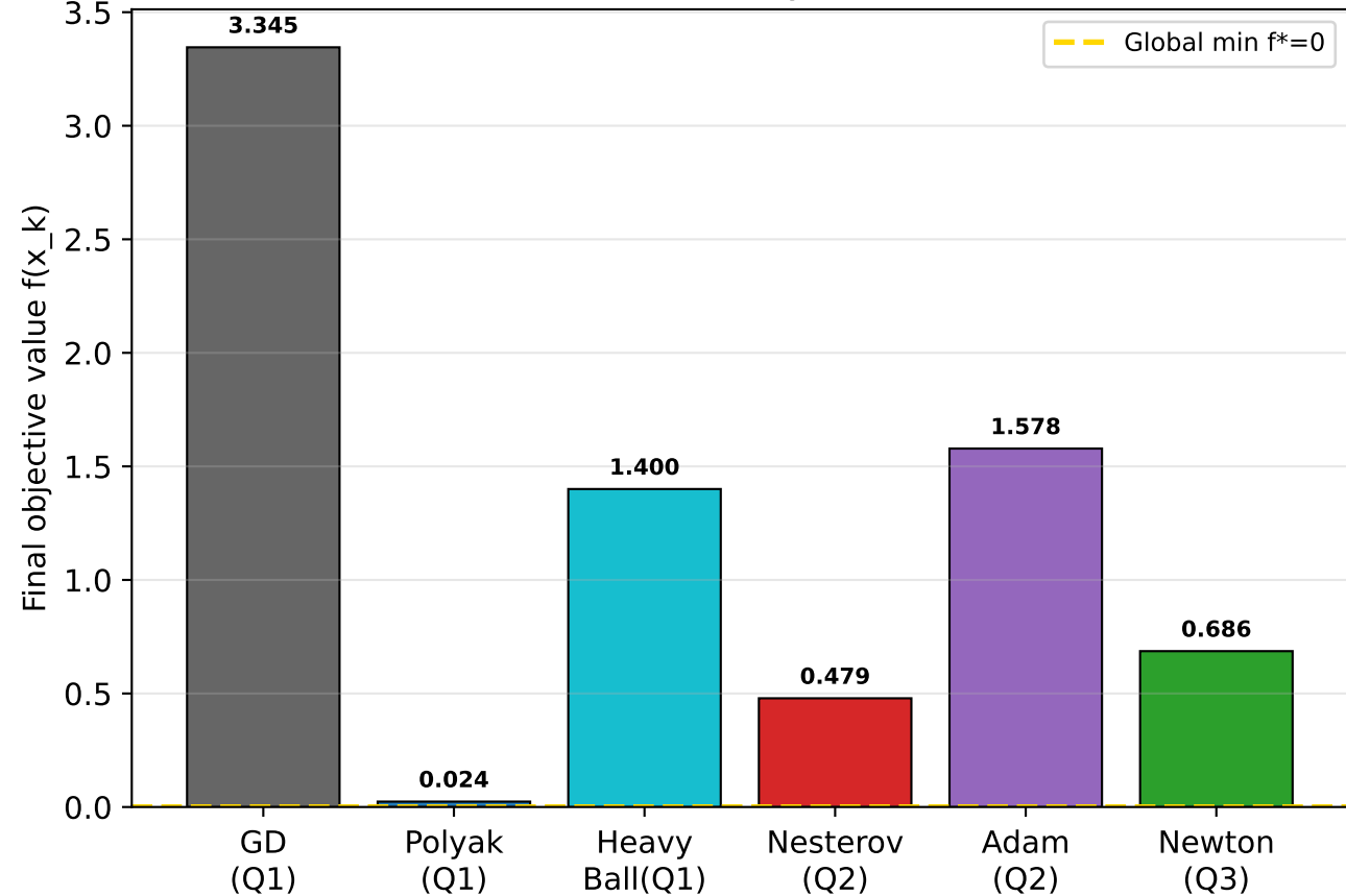
Benchmark C: Final Values by Method and Question
