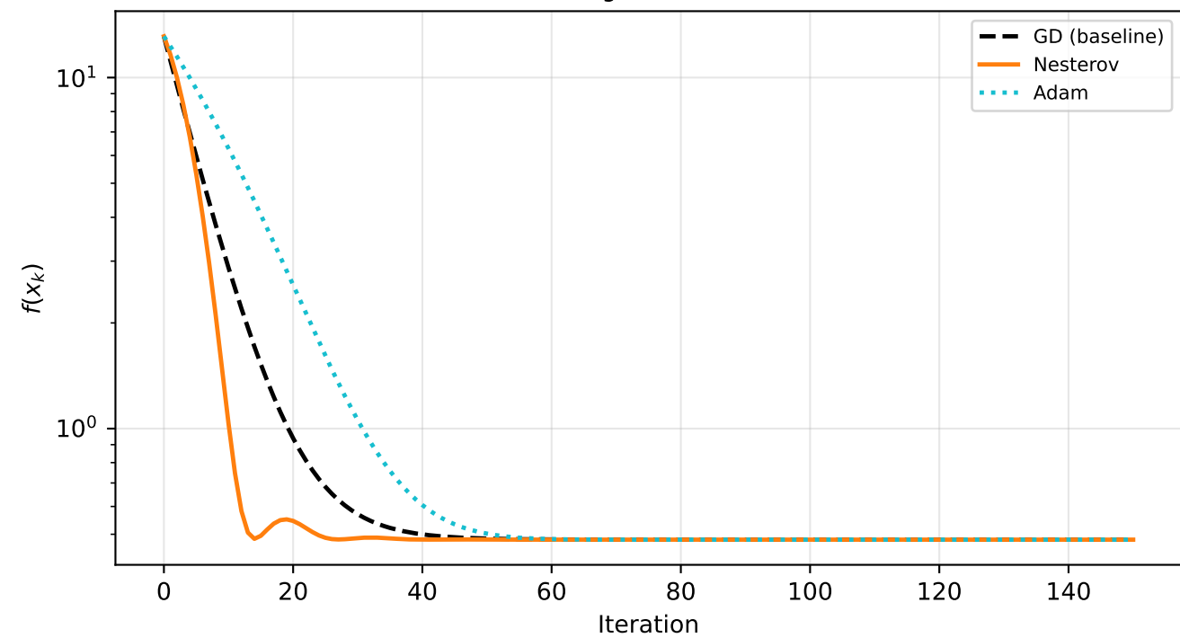
Benchmark B (Toy NN) — Q2 Methods
