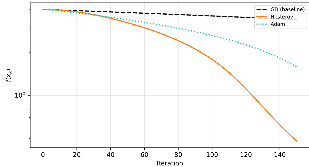
Benchmark C (Rosenbrock) — Q2 Methods
