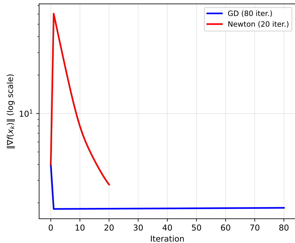
Bench. C: Rosenbrock ( \kappa \approx 2508 )
