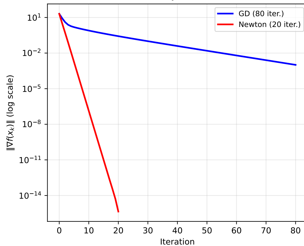
Bench. B: Toy NN ( \kappa \approx 6.90 )
