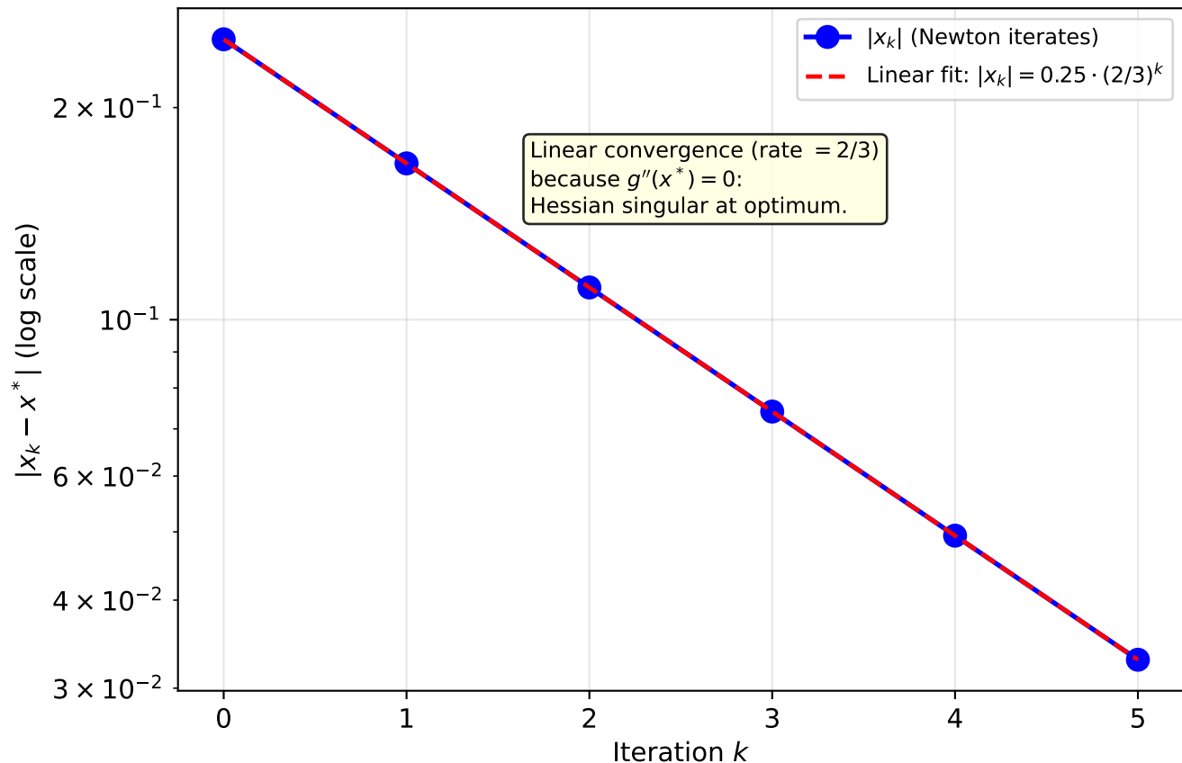
Convergence Rate: Newton on g(x) = x^4
