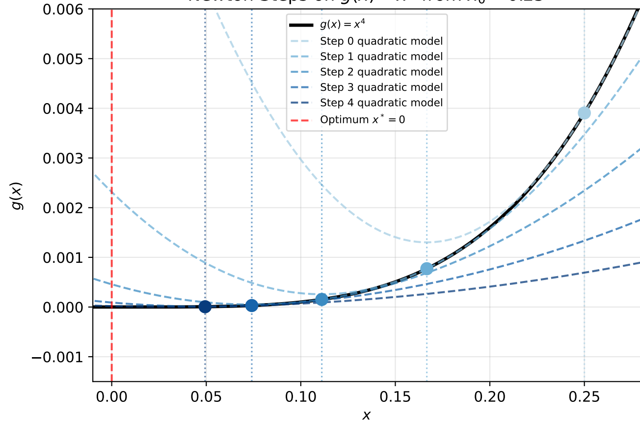
Newton Steps on g(x) = x^4 from x_0 = 0.25
