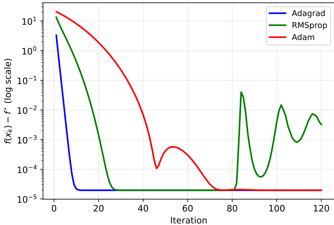
Convergence: Adagrad vs RMSprop vs Adam (Benchmark B)
