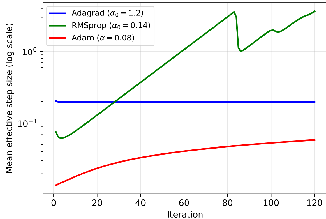
Effective Step Size Evolution on Benchmark B
