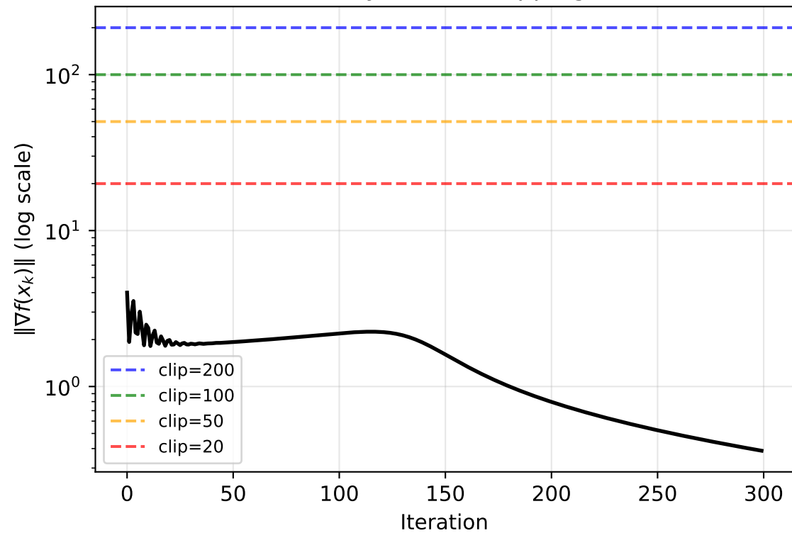
Gradient Norm Evolution (Heavy Ball, no clipping)
