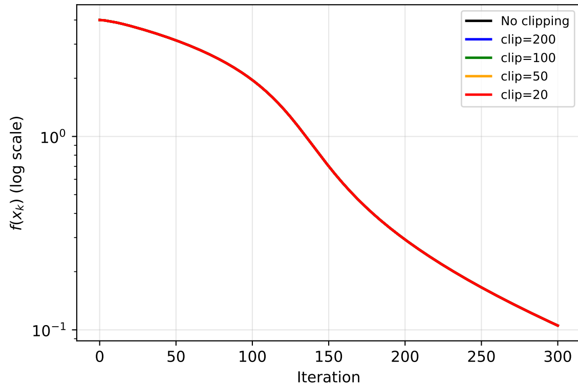
Gradient Clipping Effect on Heavy Ball (Benchmark C)
