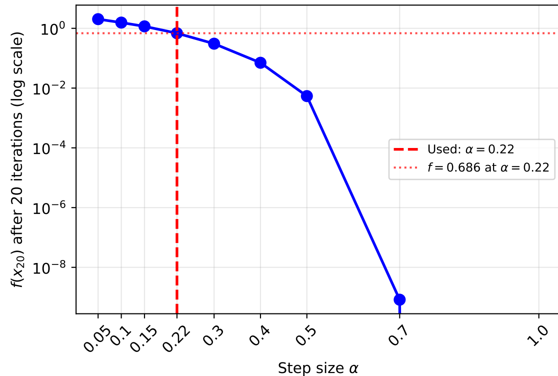
Final Objective vs. Newton Step Size (20 iterations, Rosenbrock)
