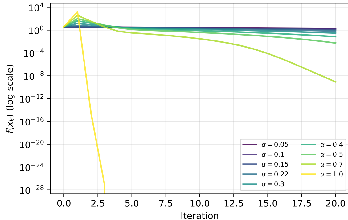
Newton Convergence on Rosenbrock for Different Step Sizes \alpha
