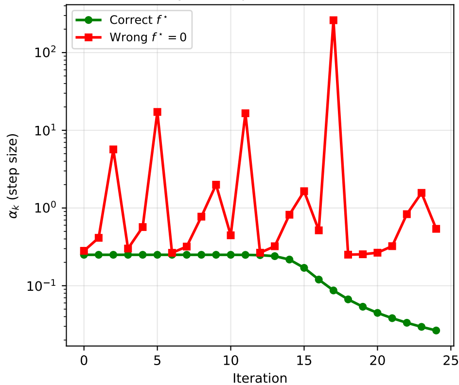
Polyak: Step Size Evolution
