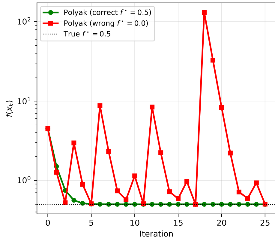
Polyak: Convergence (1D example)
