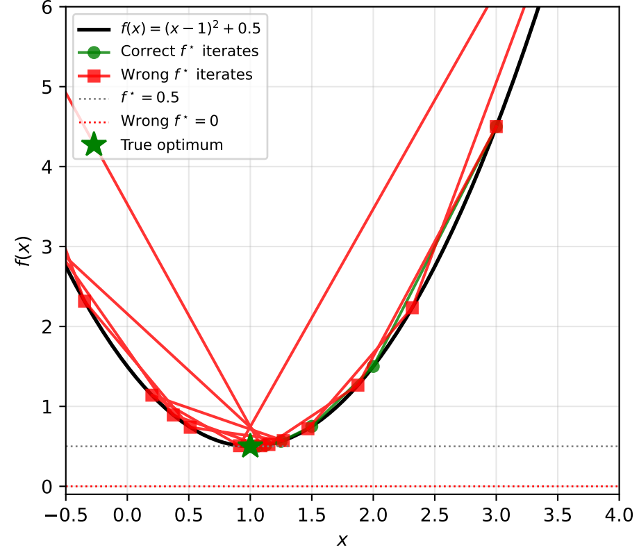
Polyak: Iterate Paths on f(x)
