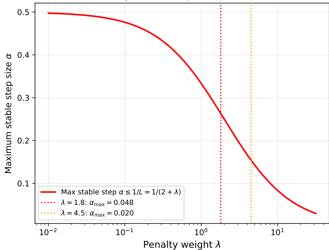
Penalty Method Step-Size Restriction
