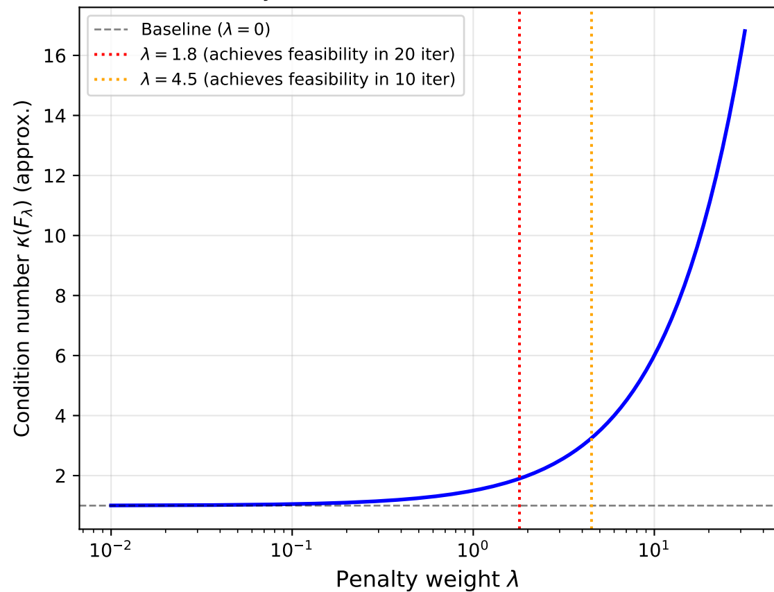
Penalty Method Condition Number Growth
