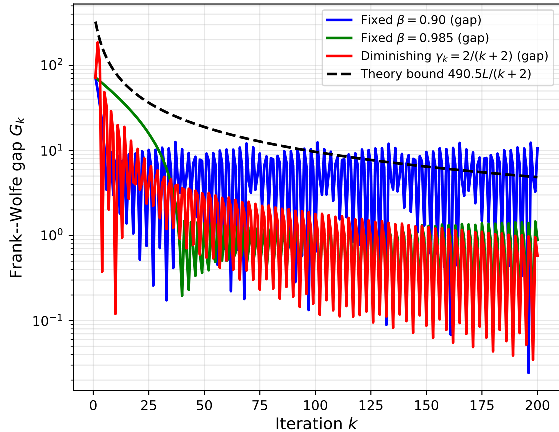
Frank--Wolfe Gap: Fixed vs Diminishing Schedule
