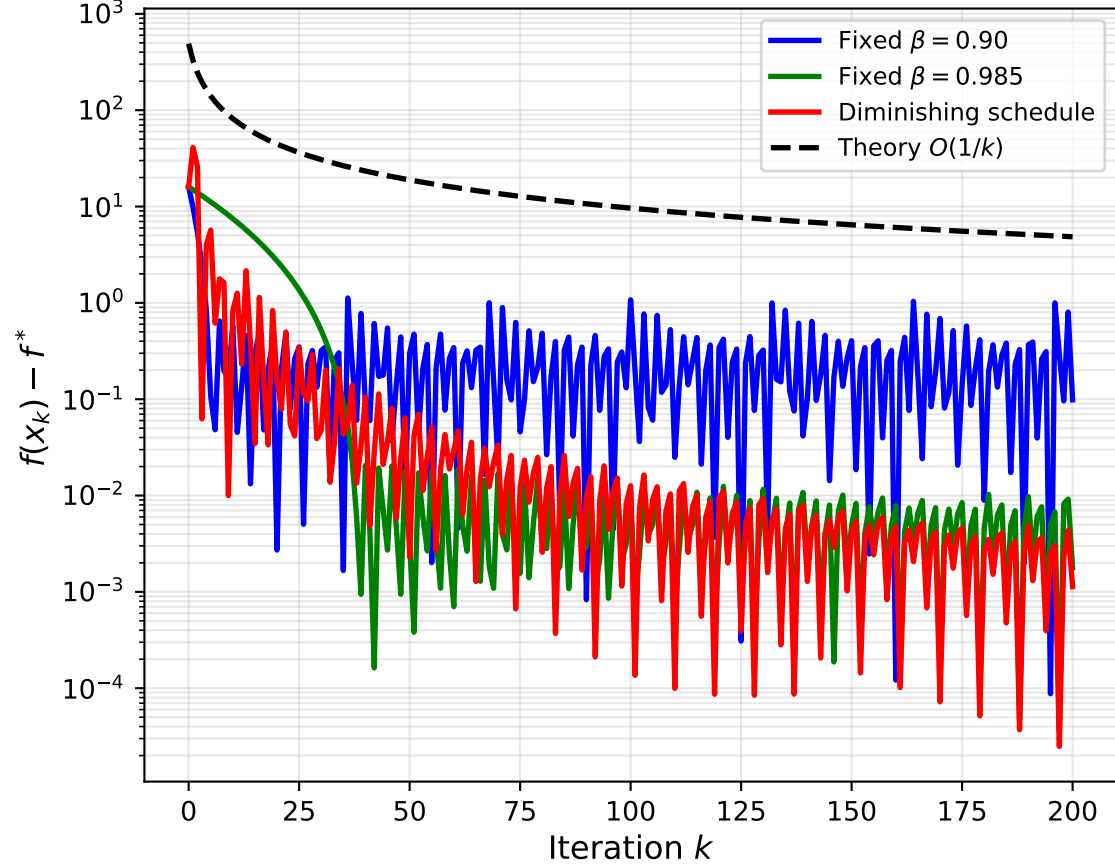
Sub-optimality: Fixed vs Diminishing Schedule
