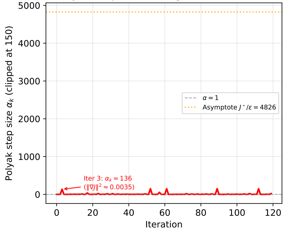
Polyak Step-Size Divergence Mechanism
