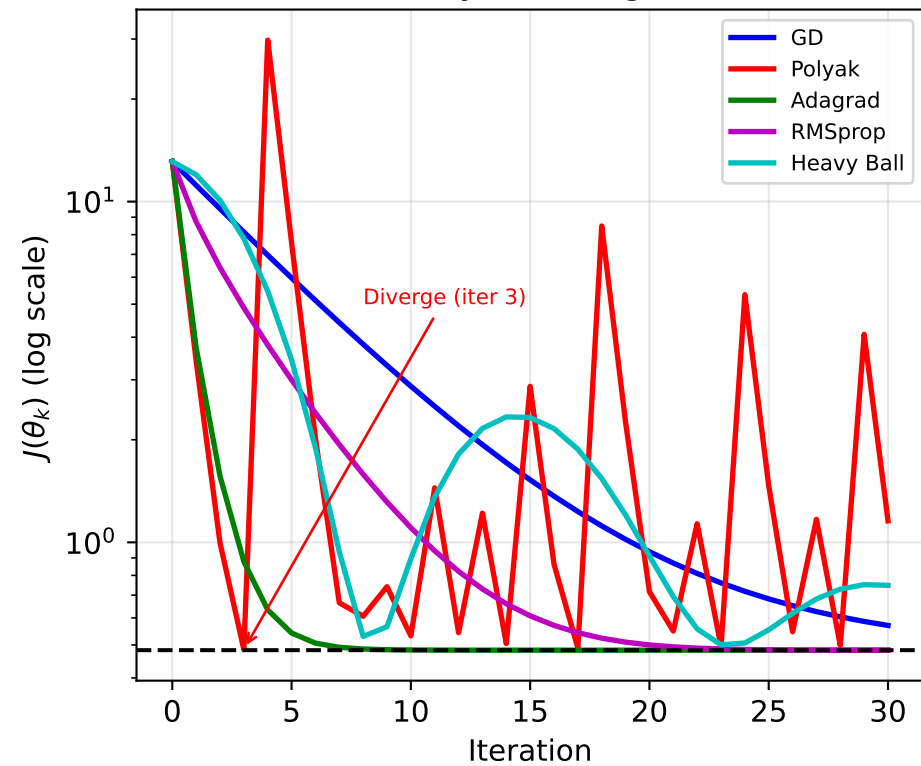
First 30 Iters (Polyak divergence at iter 3)
