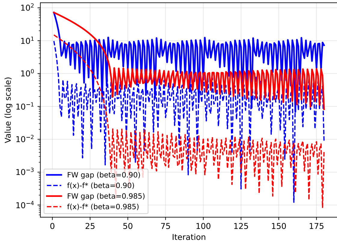
FW Gap as Upper Bound on Optimality Gap
