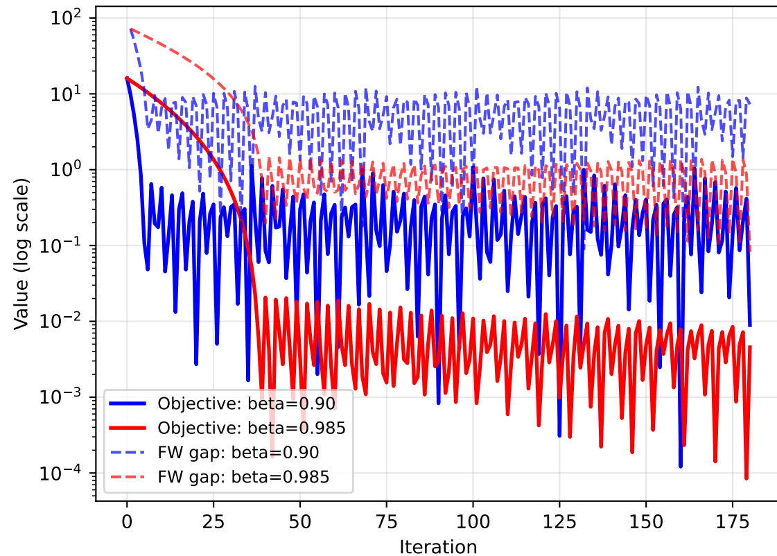
Objective vs FW Gap (Interior Optimum)
