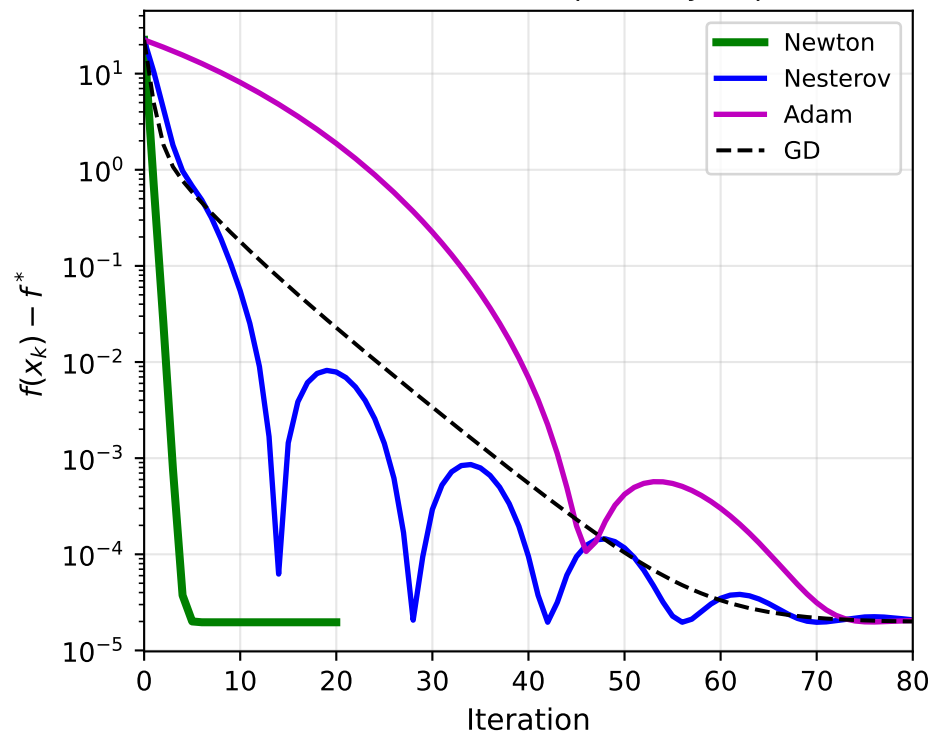
Benchmark B: Suboptimality Gap
