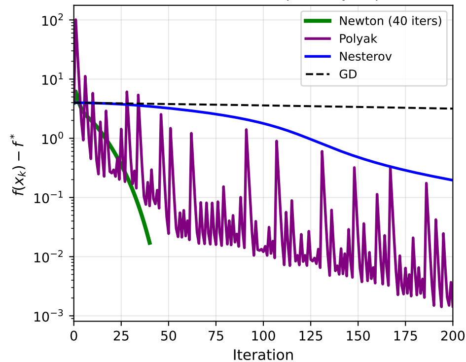
Benchmark C: Suboptimality Gap
