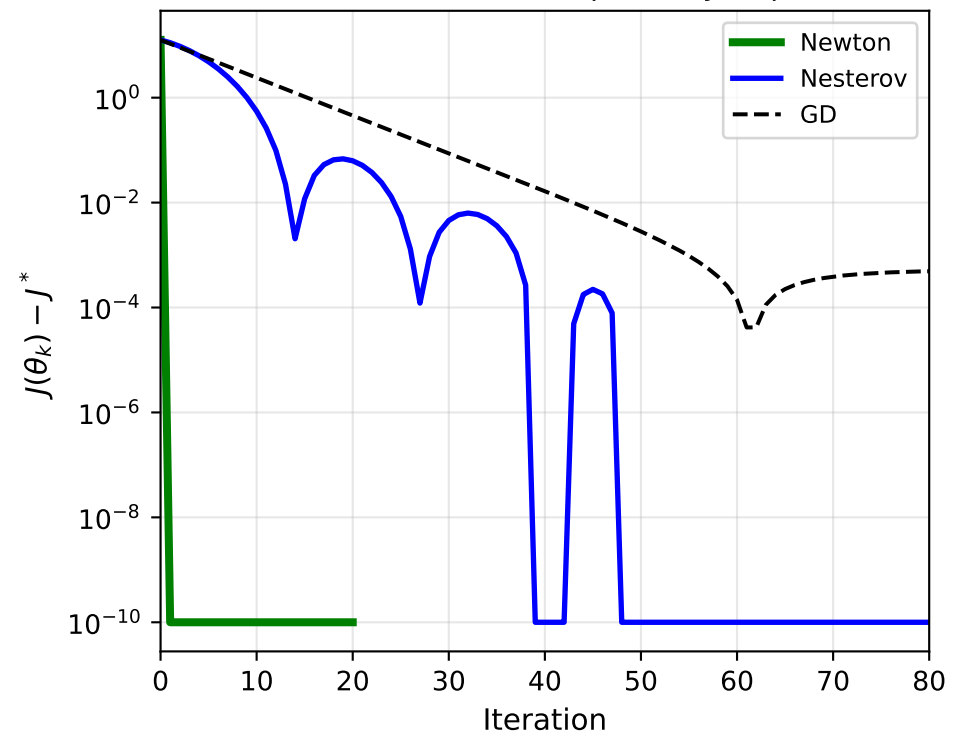
Benchmark A: Suboptimality Gap
