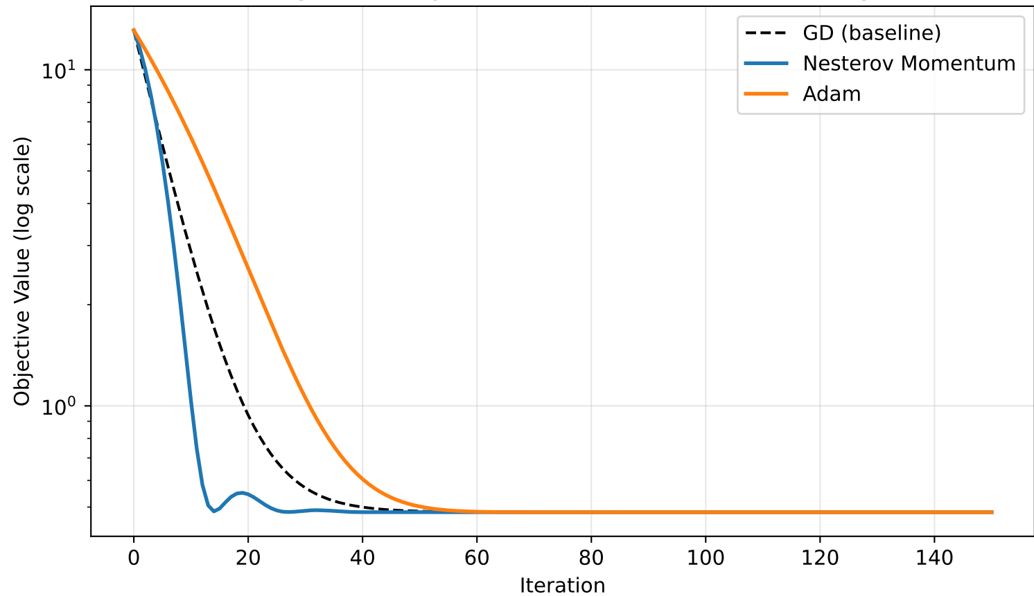
Q2: Convergence Comparison — Benchmark A (Linear Regression)
