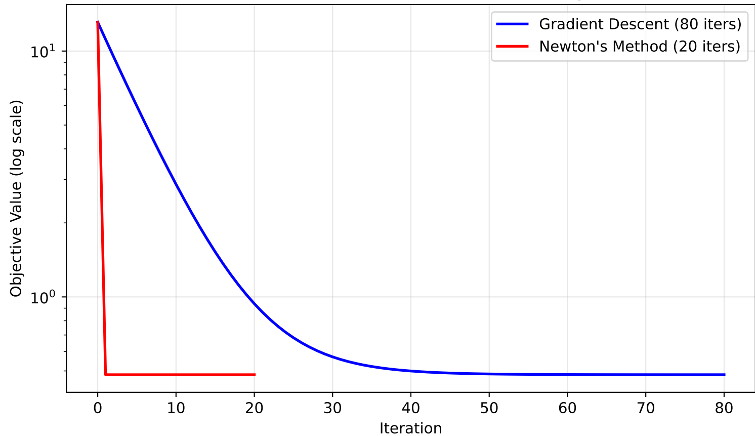
Q3: Newton vs GD — Benchmark A (Linear Regression)
