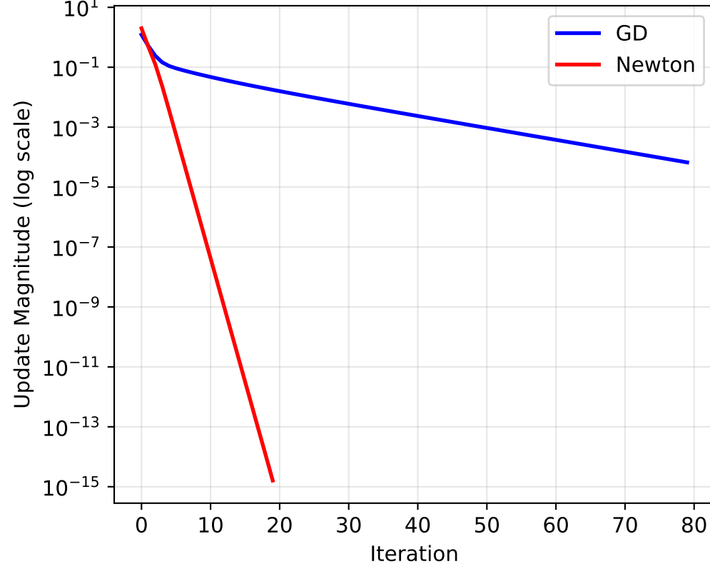
Benchmark B (Toy NN)
