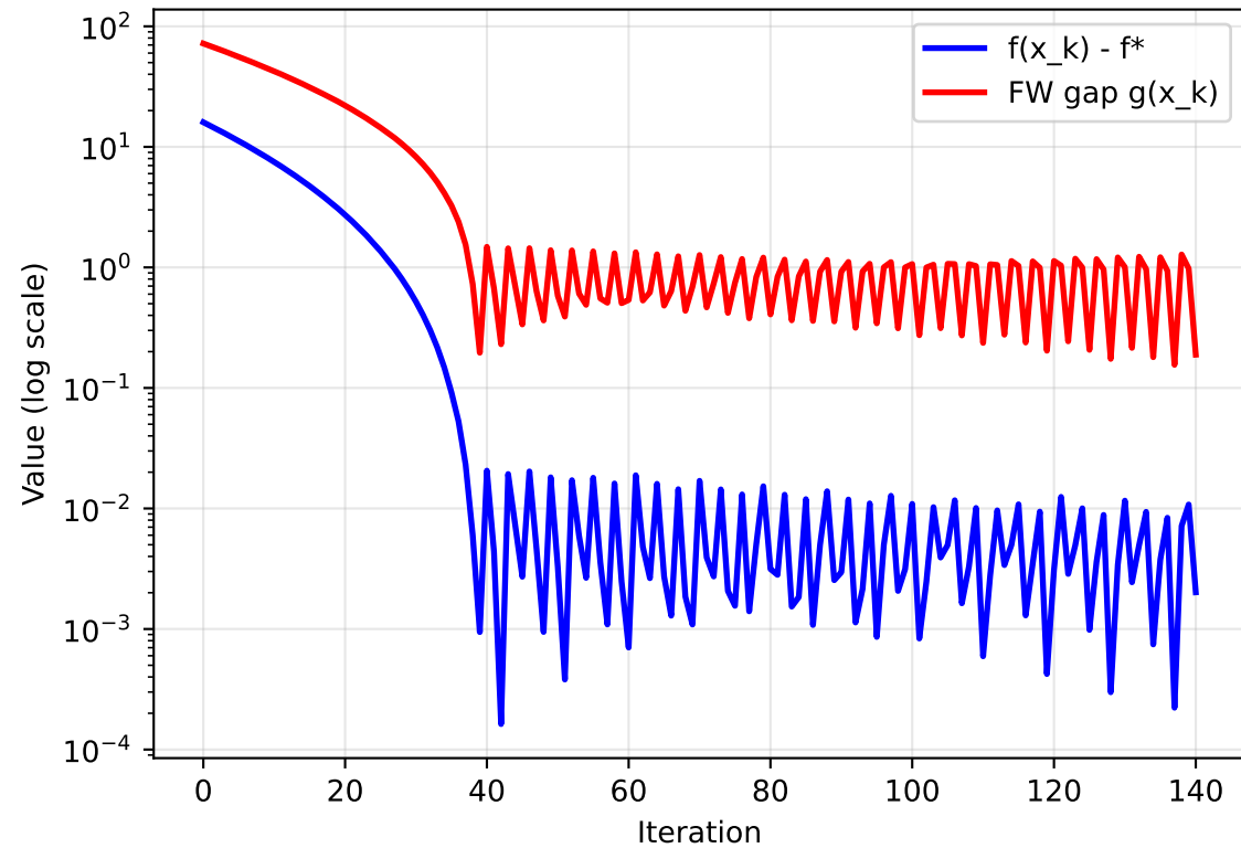
Q6: Frank-Wolfe gap as convergence certificate
