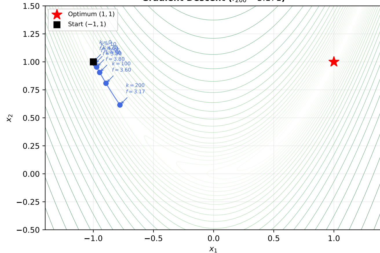
Gradient Descent ( f_{200} = 3.171 )
