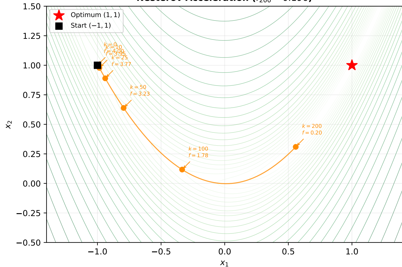
Nesterov Acceleration ( f_{200} = 0.196 )
