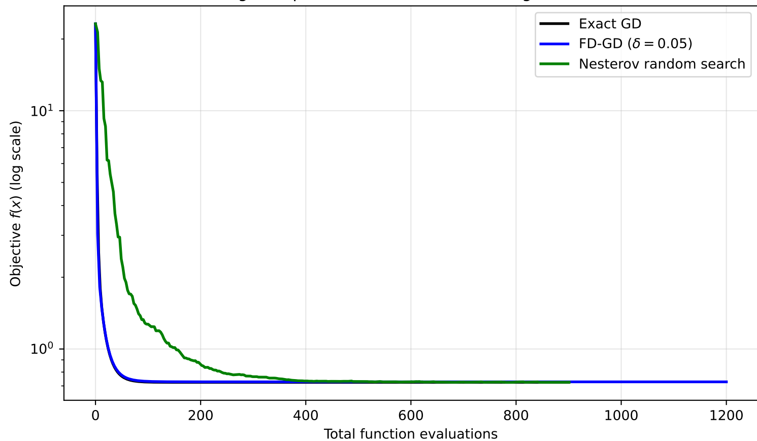
Q4: Convergence per Function Evaluation Budget (Benchmark B)
