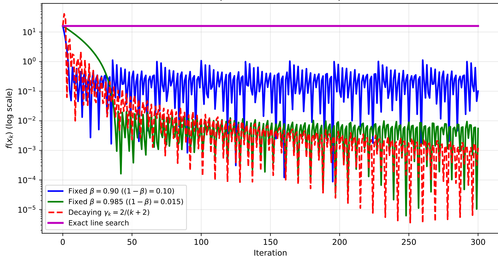
Q6-II: Frank--Wolfe Step Schedules — Interior Optimum (300 iters)
