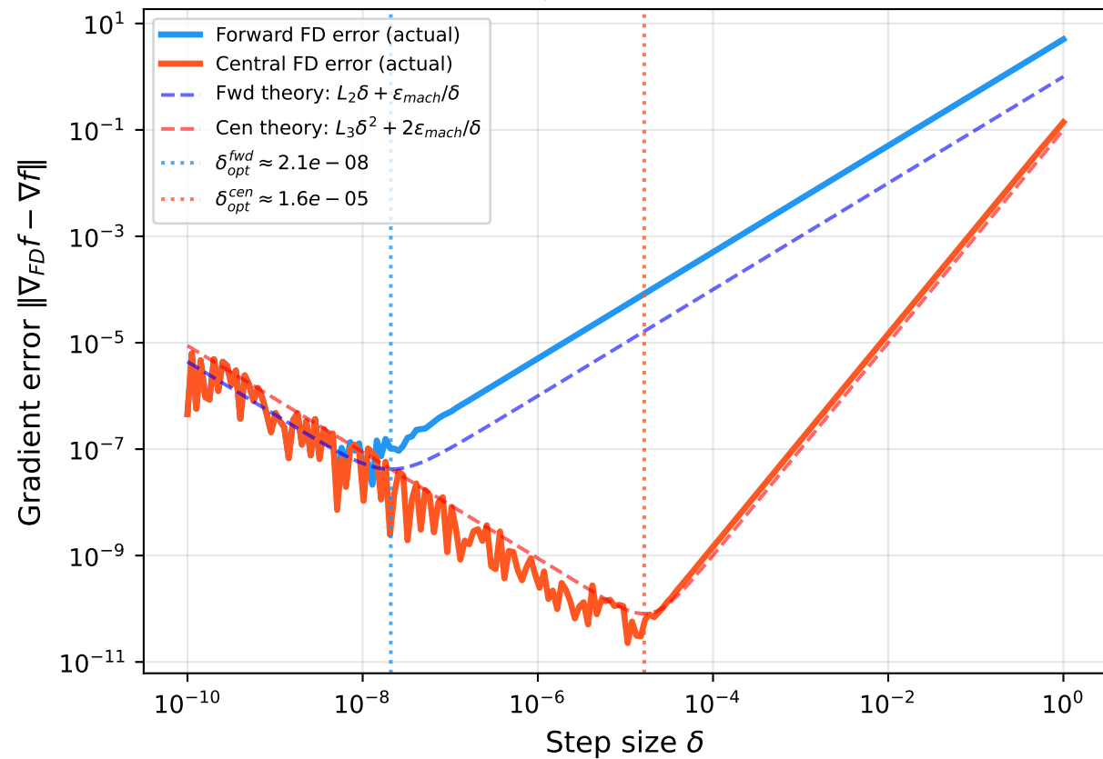
Forward vs Central Finite Differences Error Decomposition on Benchmark B
