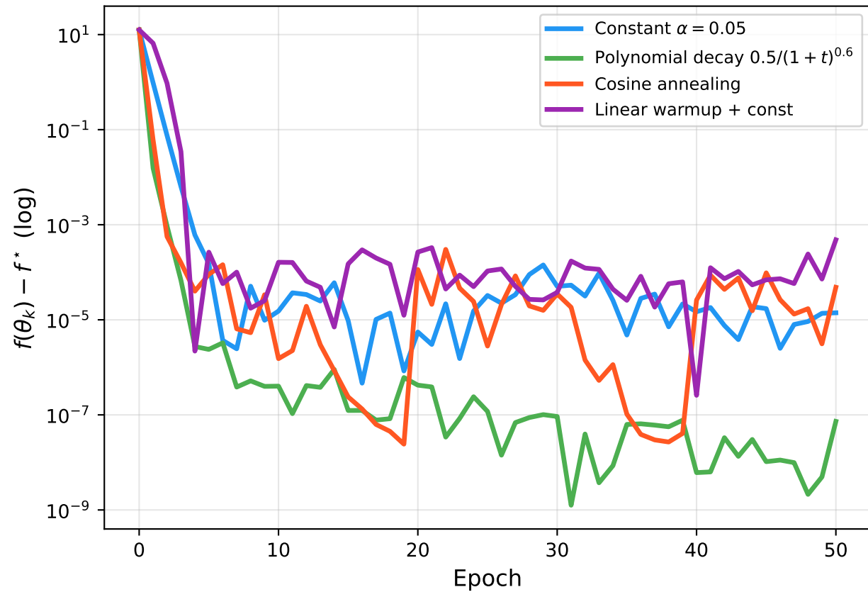
SGD Learning Rate Schedules (Benchmark A, batch=40)
