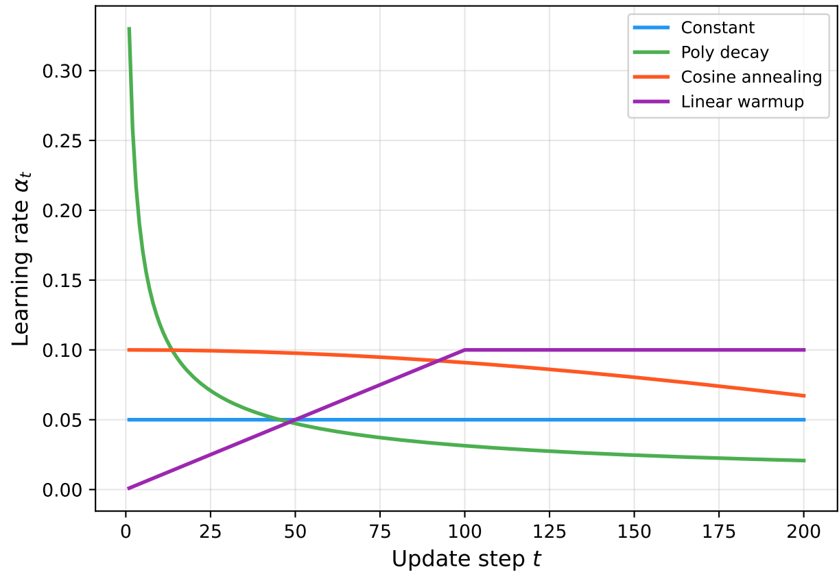
Learning Rate Schedules (first 200 steps) Showing Schedule Shape
