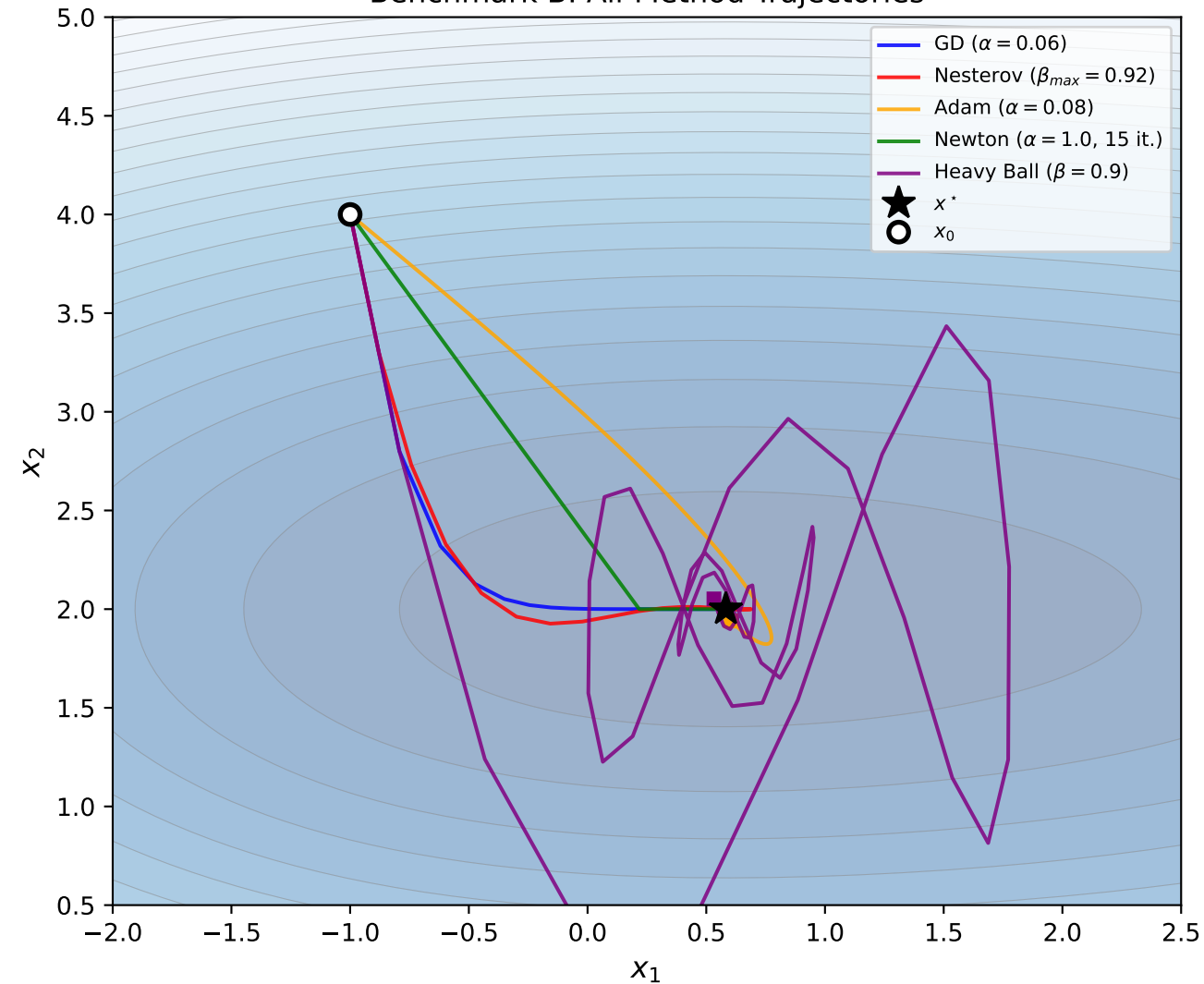
Benchmark B: All-Method Trajectories
