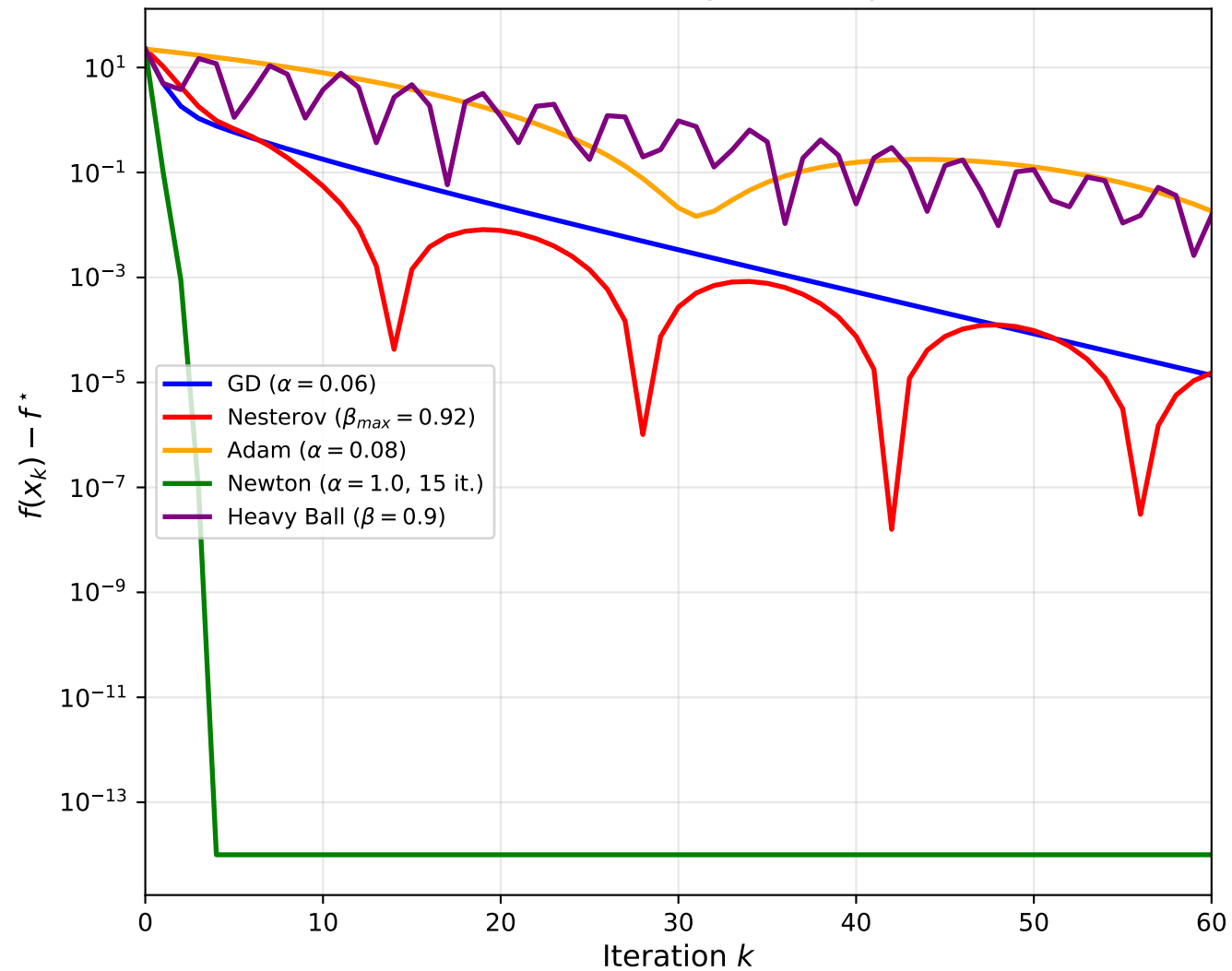
Benchmark B: Convergence Comparison
