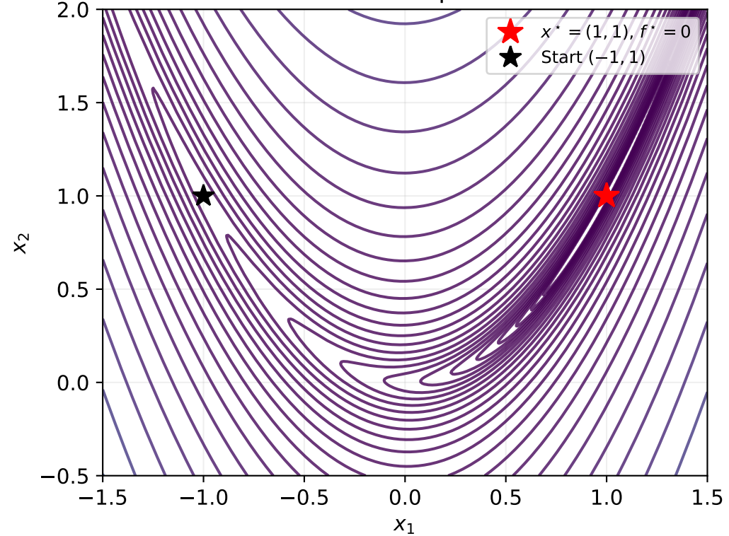
Benchmark C: Rosenbrock
