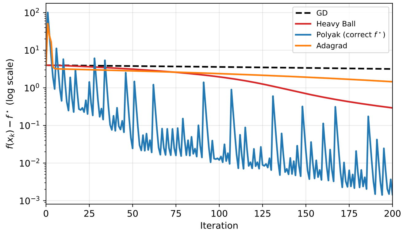
Q1: Convergence Gap — Benchmark C (Rosenbrock, f^* = 0 )
