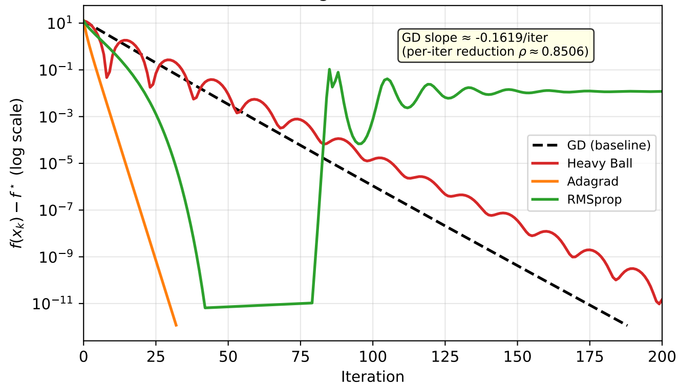
Q1: Convergence Gap — Benchmark A (Linear Regression, f^* \approx 0.4826 )
