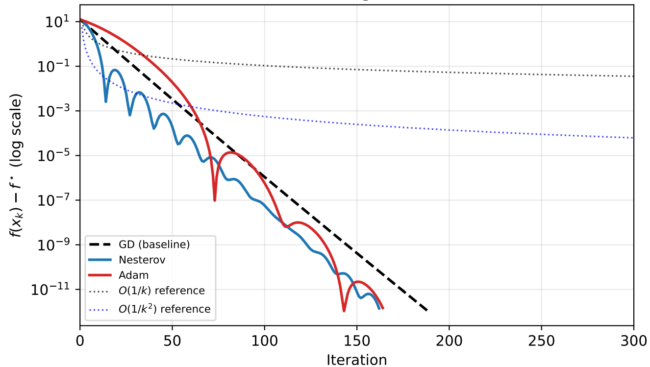
Q2: Acceleration — Benchmark A (Linear Regression)
