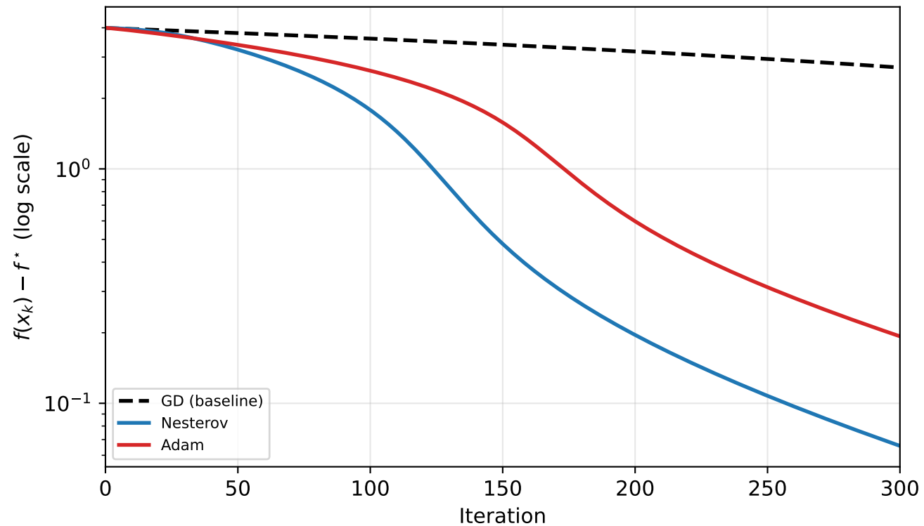
Q2: Acceleration — Benchmark C (Rosenbrock, f^* = 0 )
