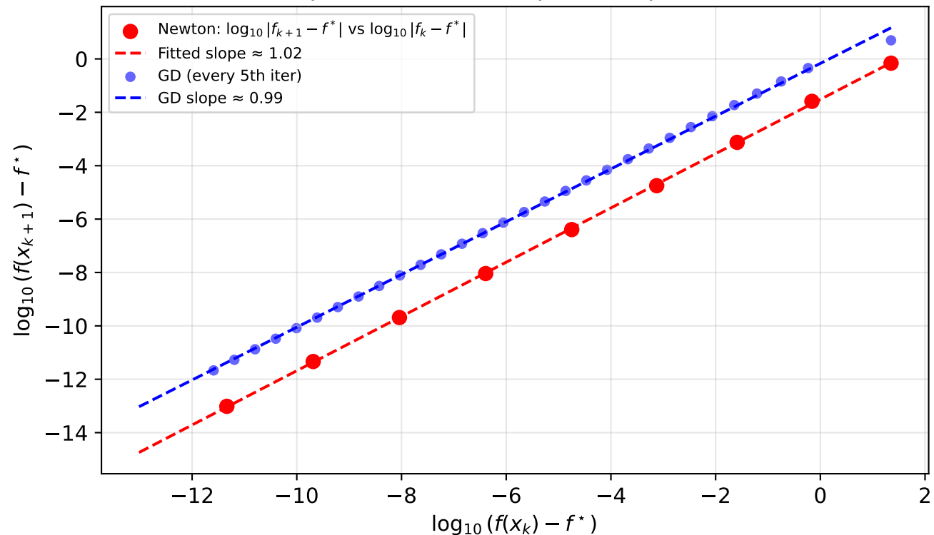
Q3: Convergence Order Analysis (Slope \approx 1 : linear; Slope \approx 2 : quadratic)
