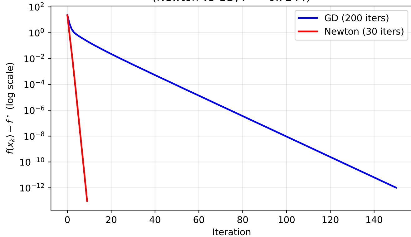
Q3: Convergence Gap — Benchmark B (Newton vs GD, f^* \approx 0.7244 )
