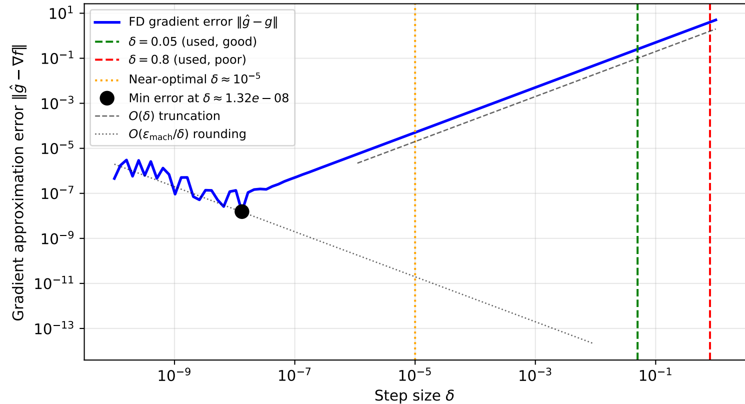
Q4: Finite Difference Error vs Step Size \delta (Benchmark B at x = (0.5, 2.5) )
