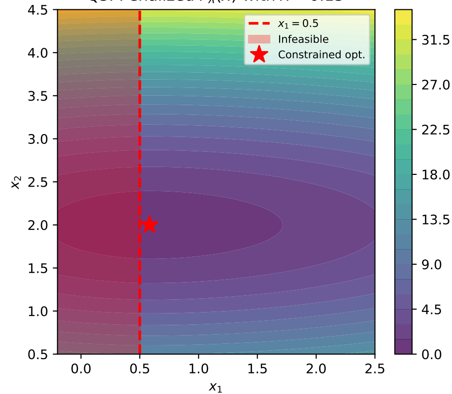
Q5: Penalized F_\lambda(x) with \lambda = 0.15
