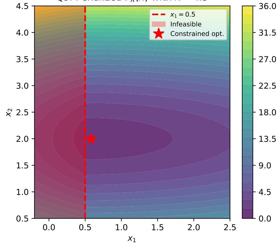
Q5: Penalized F_\lambda(x) with \lambda = 4.5
