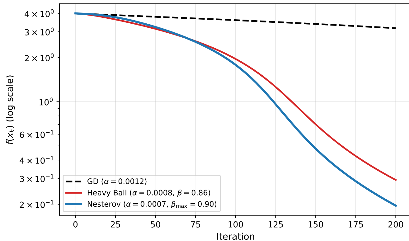
Heavy Ball vs Nesterov on Rosenbrock (200 iterations, Benchmark C)
