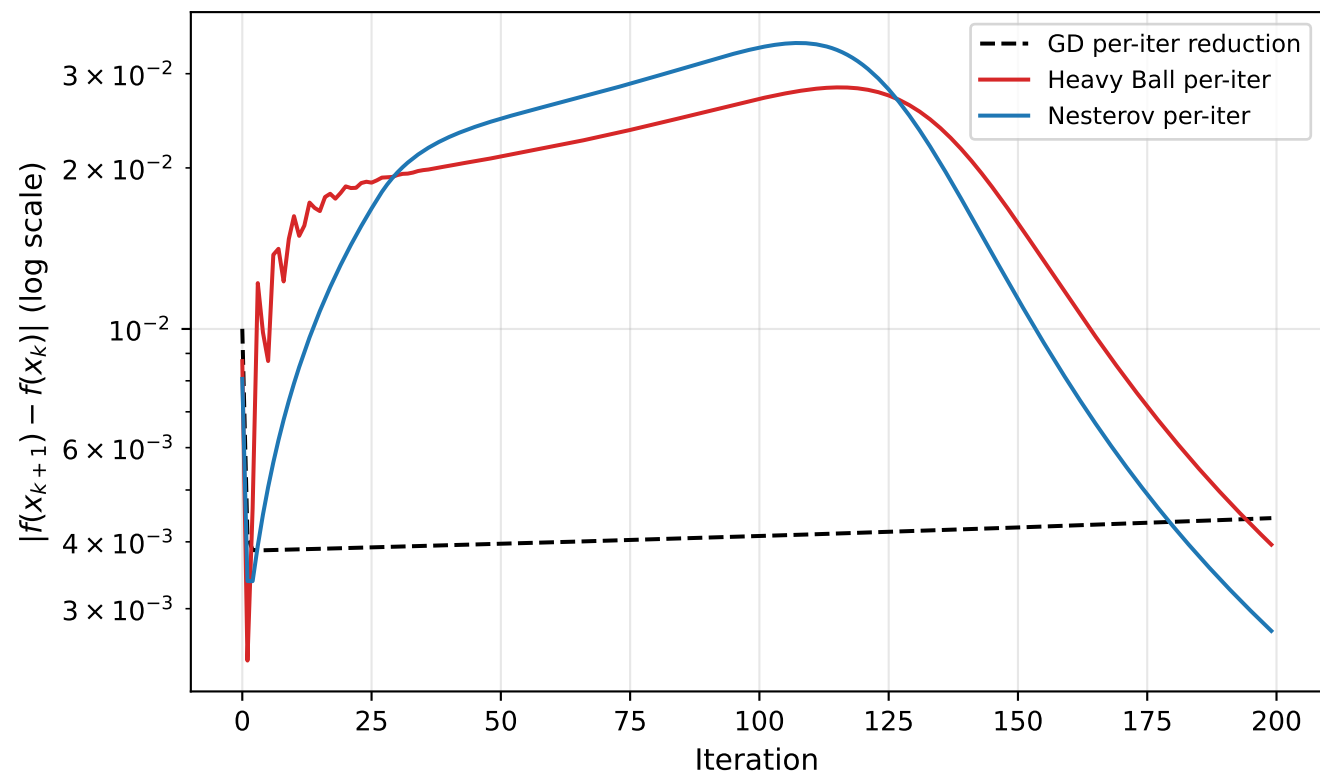
Per-Iteration Objective Reduction (Rosenbrock Benchmark C)
